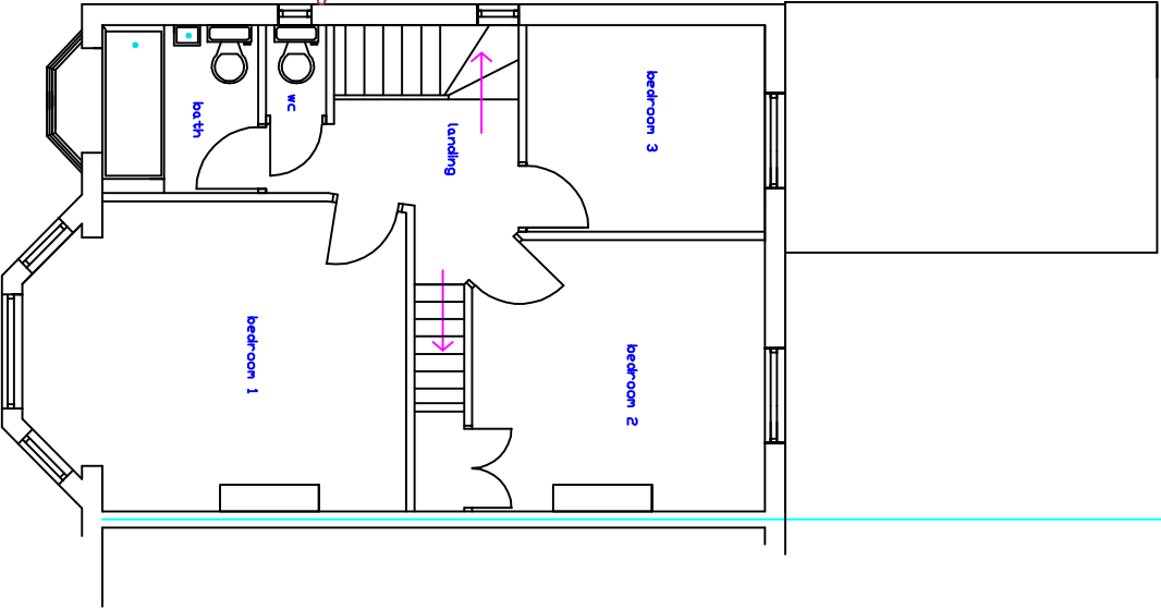
EXISTING FIRST FLOOR 1:100
