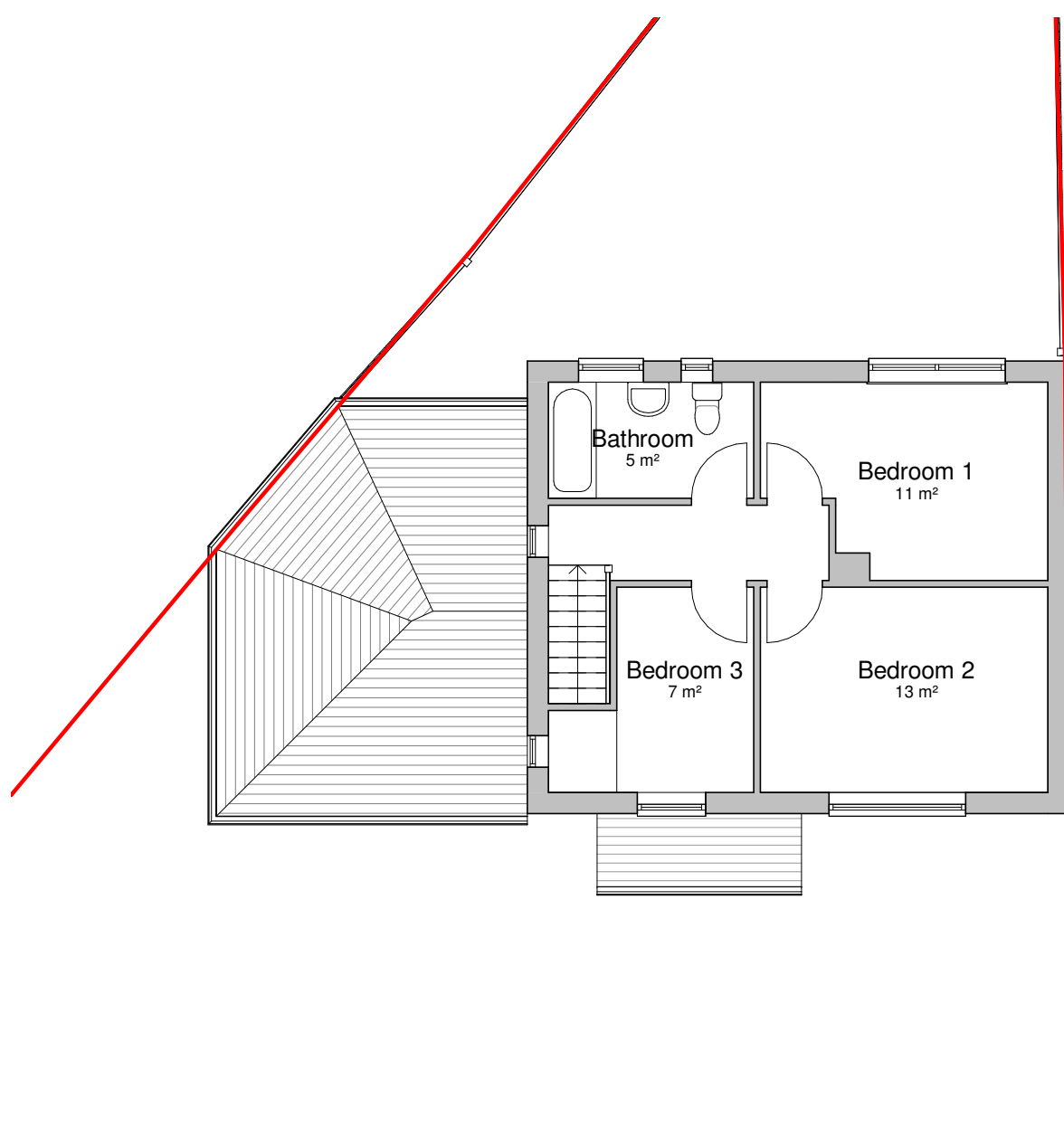
2 Existing First Floor Plan 1 : 100
