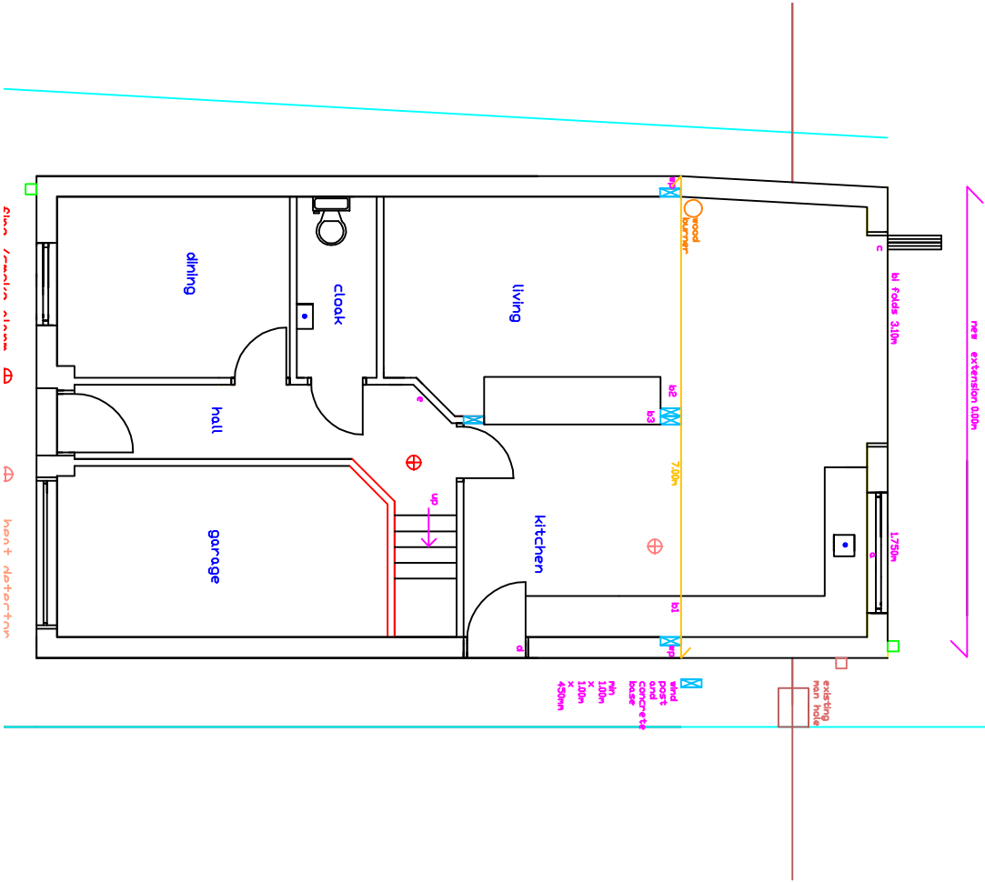
PROPOSED GROUND FLOOR LAYOUT 1:100
