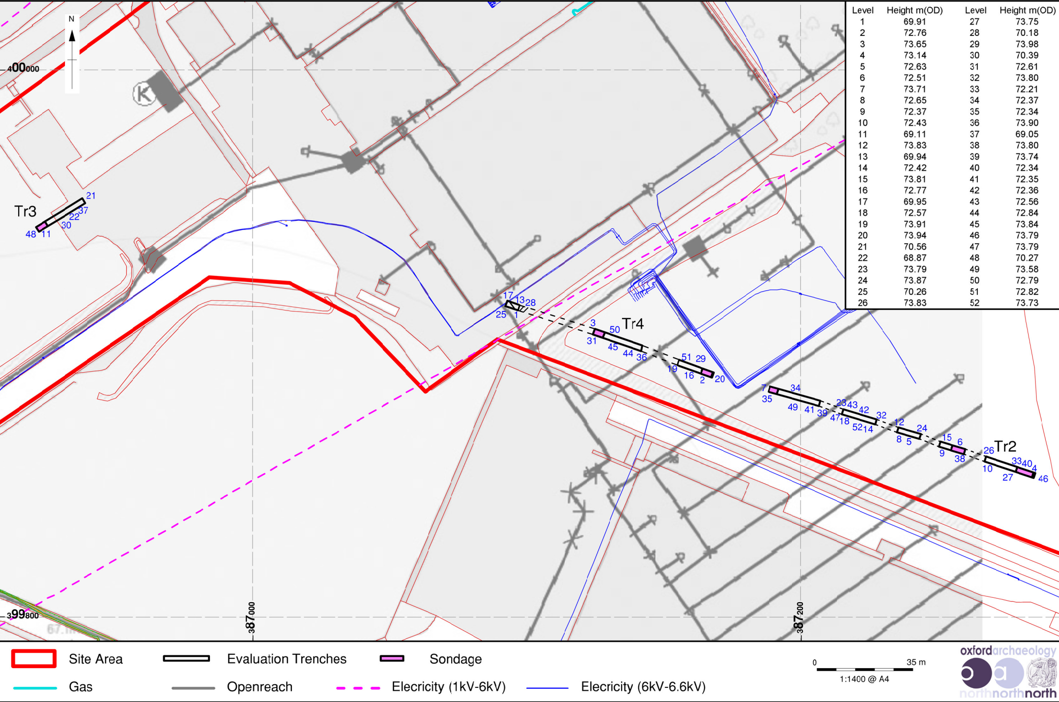
Figure 3: Plan of evaluation trenches superimposed on services
