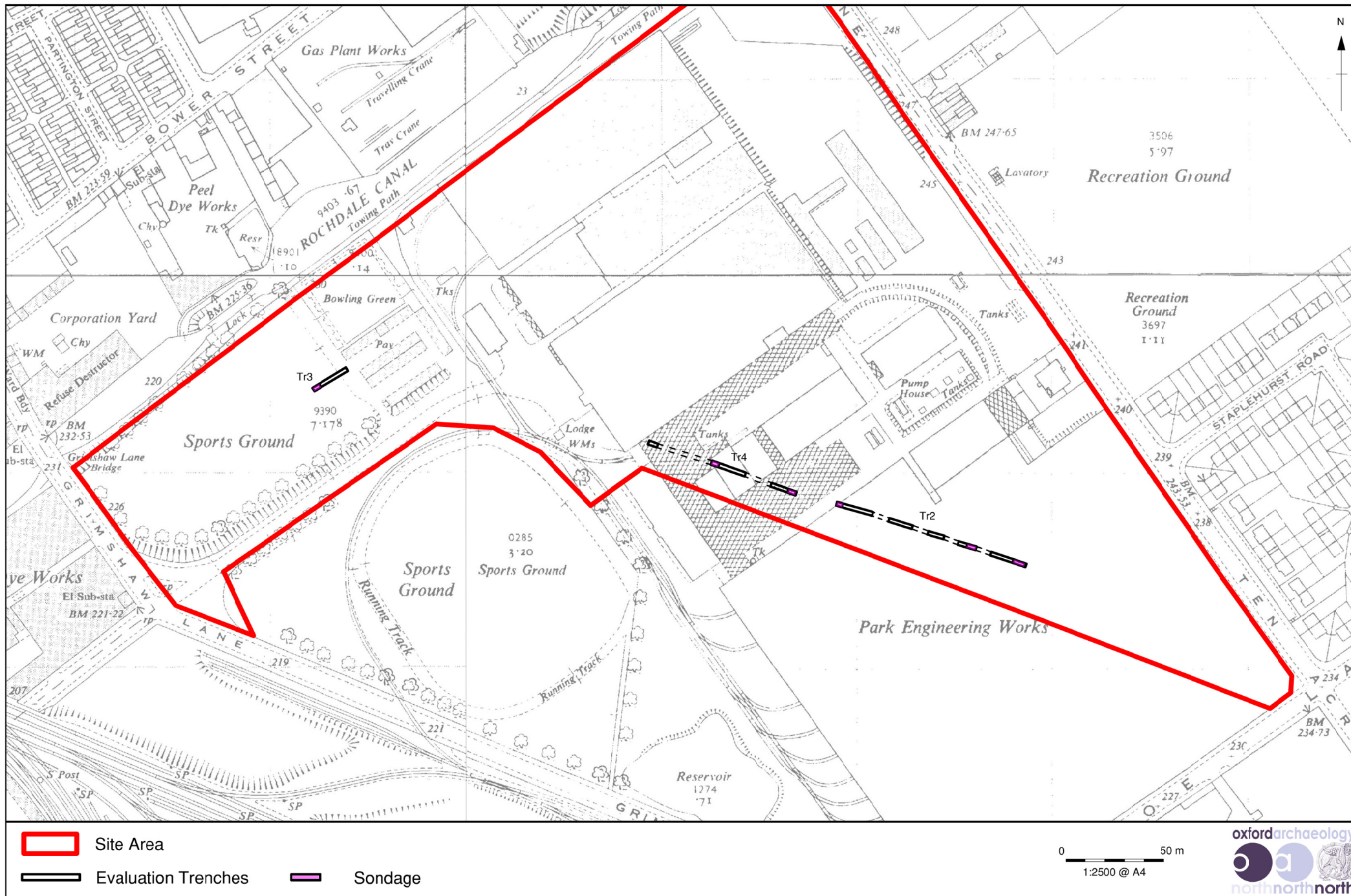
Figure 4: Evaluation trenches superimposed on the Ordnance Survey map of 1951
