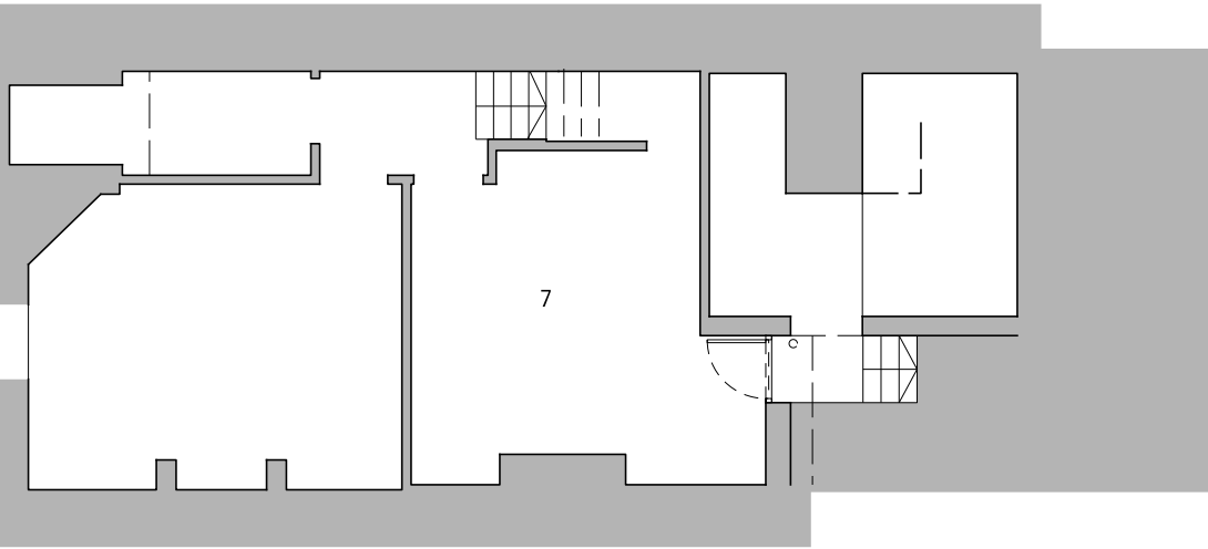
Existing basement floor plan
