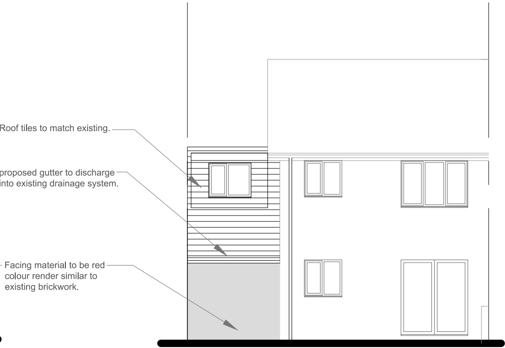
Rear Elevation
