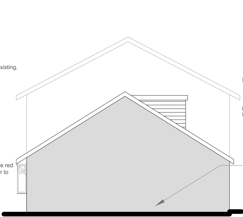
Side Elevation
