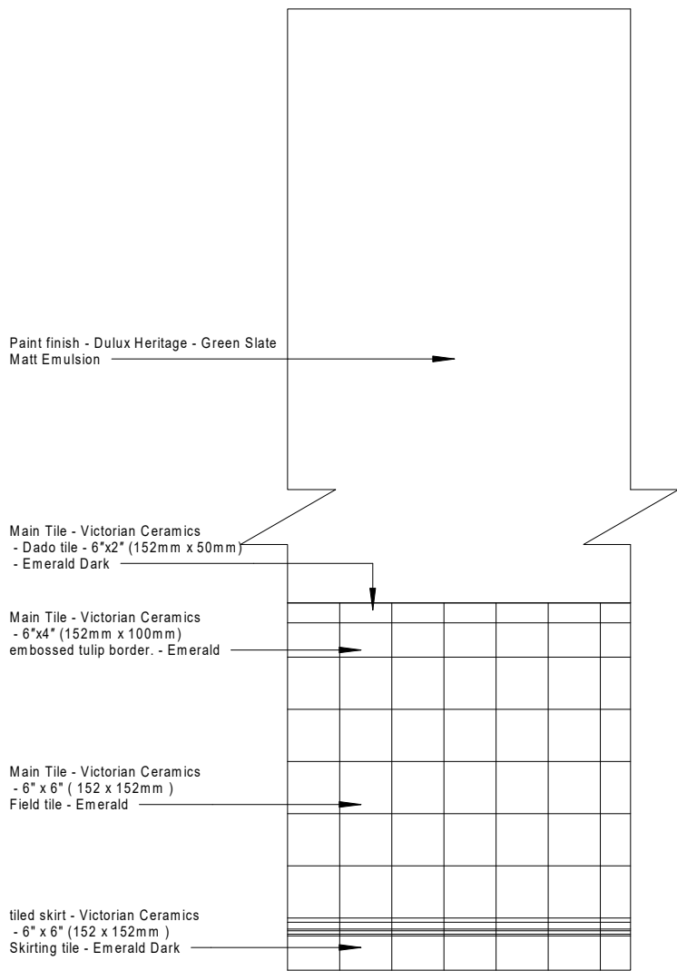
Wall Tiling and Decorations detail 1 : 20
