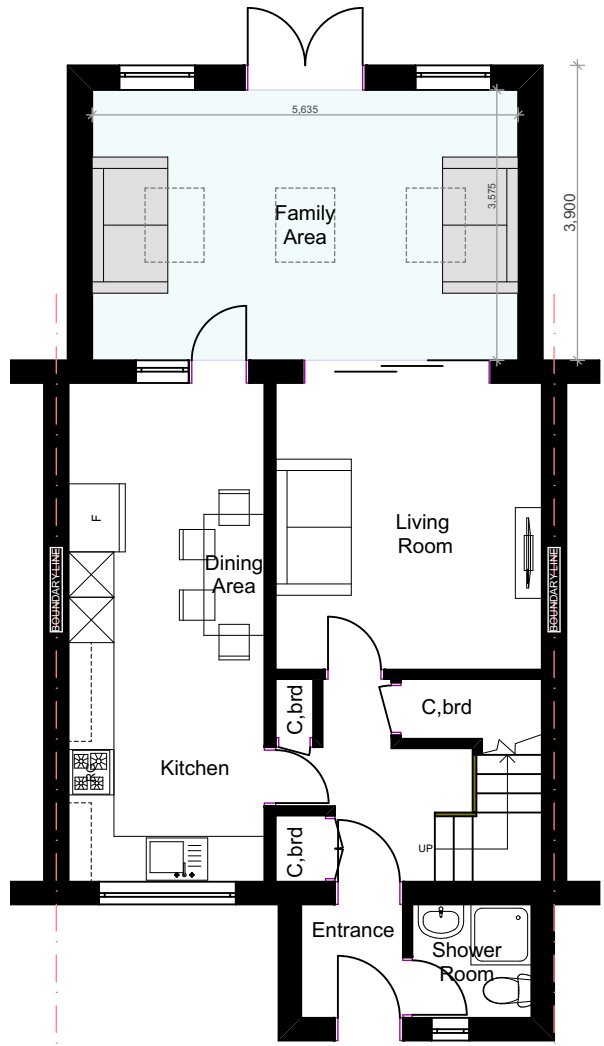
PROPOSED GA GROUND FLOOR PLAN @1:100
