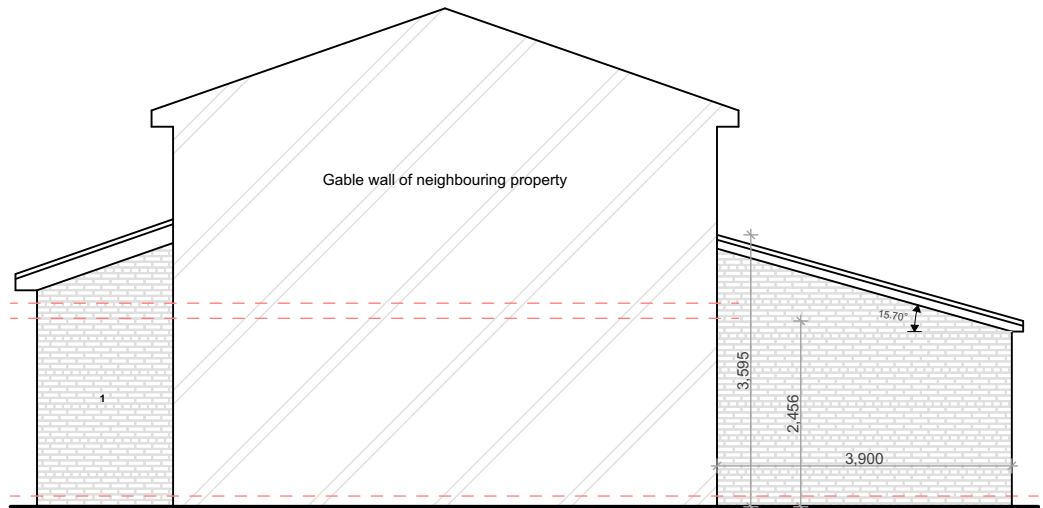
PROPOSED GA SIDE ELEVATION 1 @1:100
