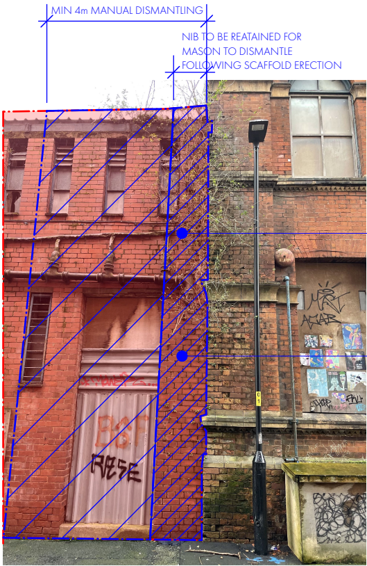
IMAGE 001- BROCK STREET - Junction between retained and demolished
