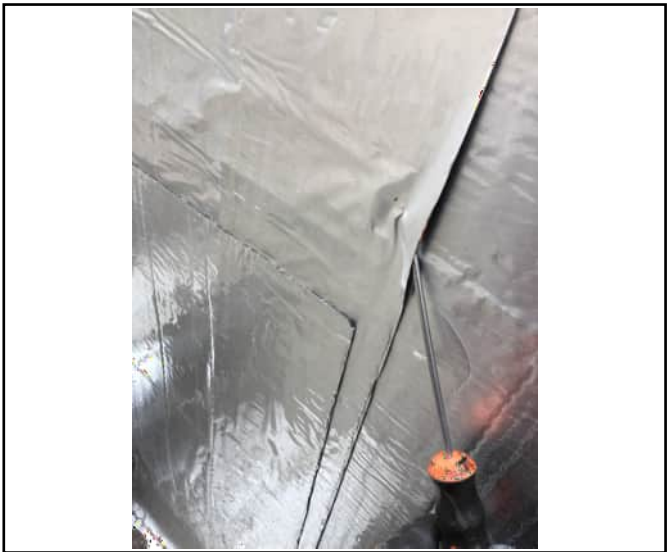
Pick and probe test to perimeter
