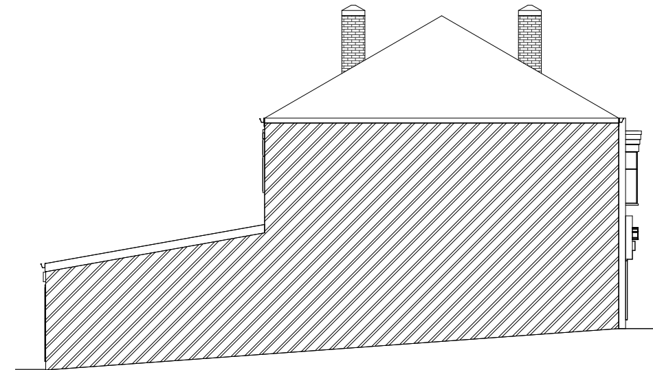
4 Existing Right Elevation 1 : 150
