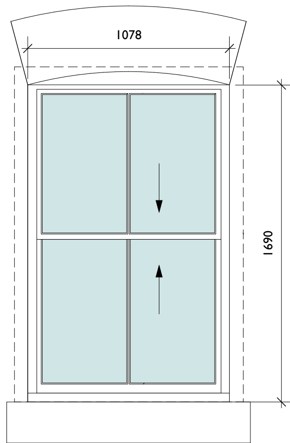
Window Type 5B - 1 No. W504 Replacement sash windows with glazing bar, both sashes opening Type A Jamb Detail
