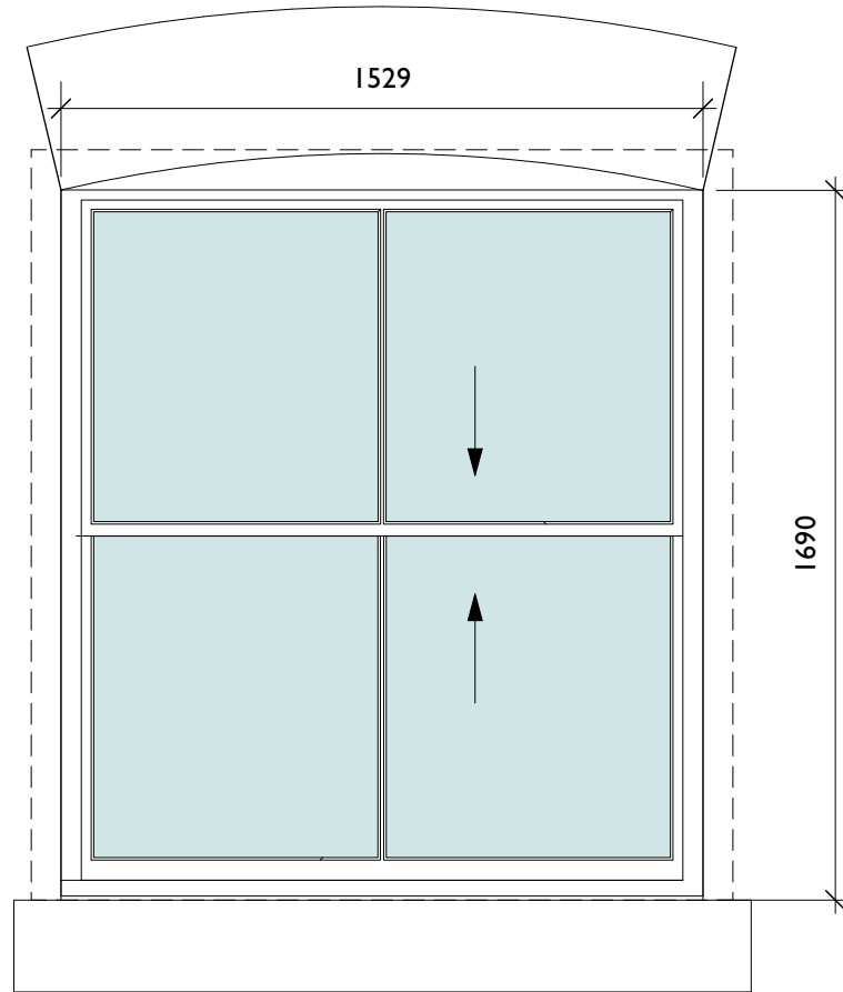
Window Type 5C - 1 No. W508 Replacement sash windows with glazing bar, both sashes opening Type A Jamb Detail
