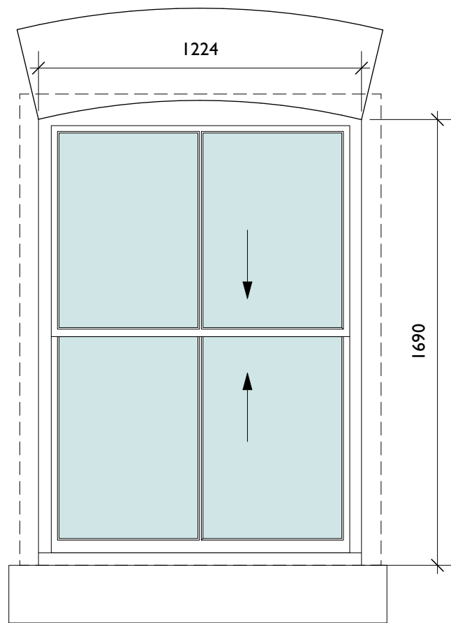
Window Type 5A - 6 No. W501, W502, W503, W505, W506 & W507 Replacement sash windows with glazing bar, both sashes opening Type A Jamb Detail
