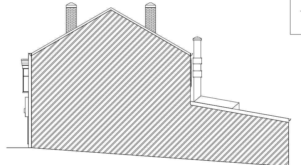
3 Proposed Left Setout 1 : 150
