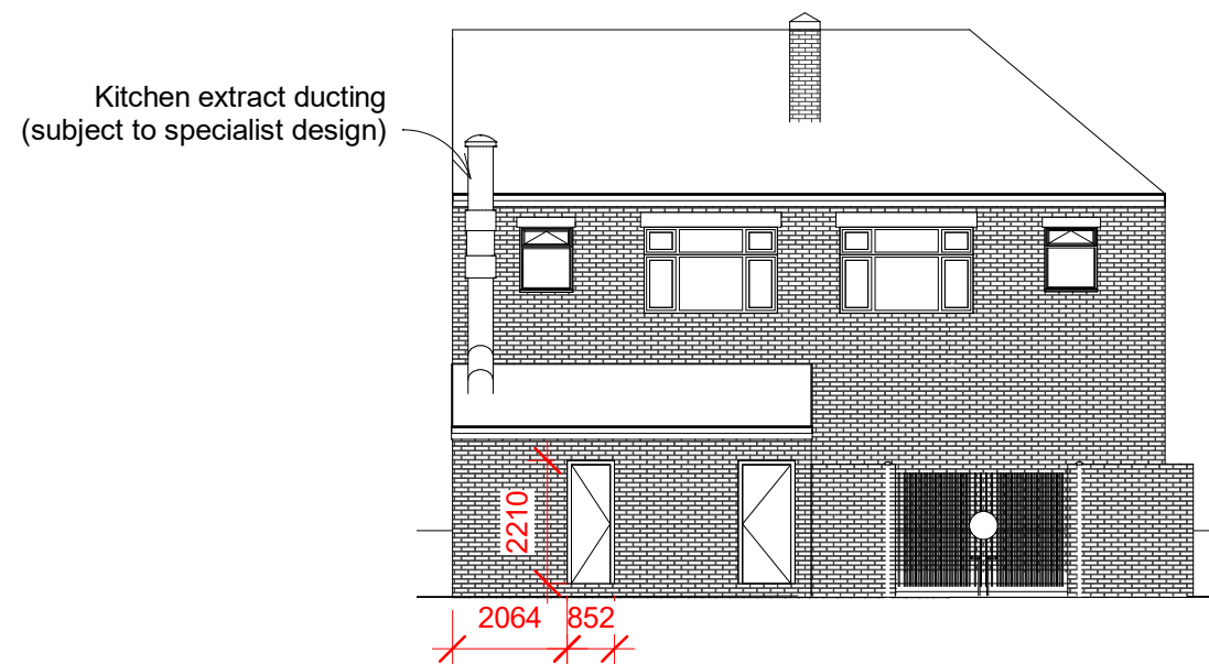
2 Proposed Rear Setout 1 : 150
