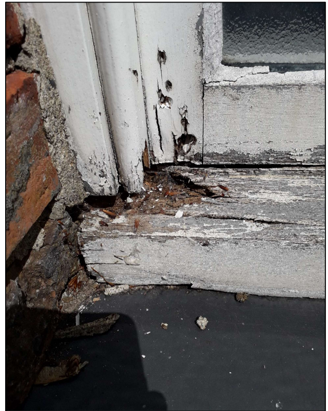
Figure 8: View of Rot to Window Cill & Sash
