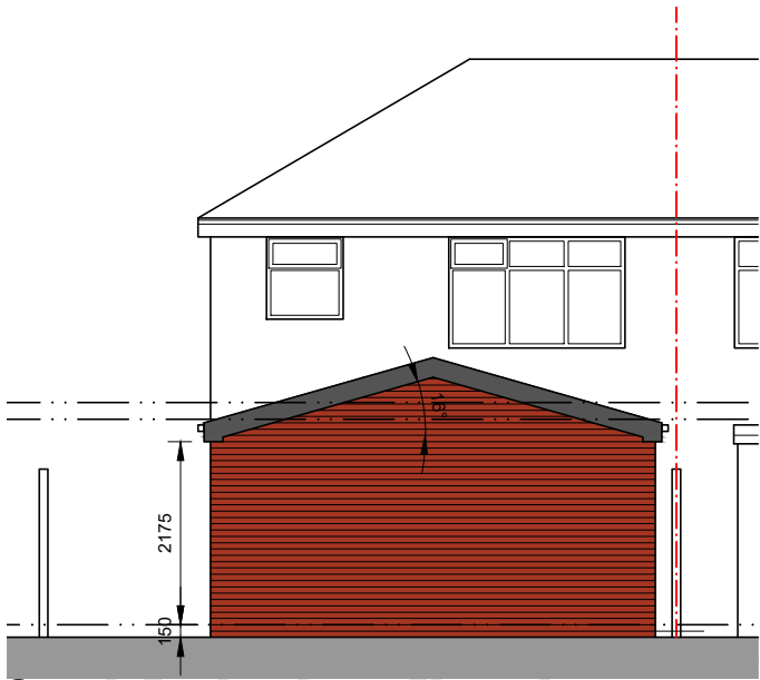
South Facing Rear Elevation
