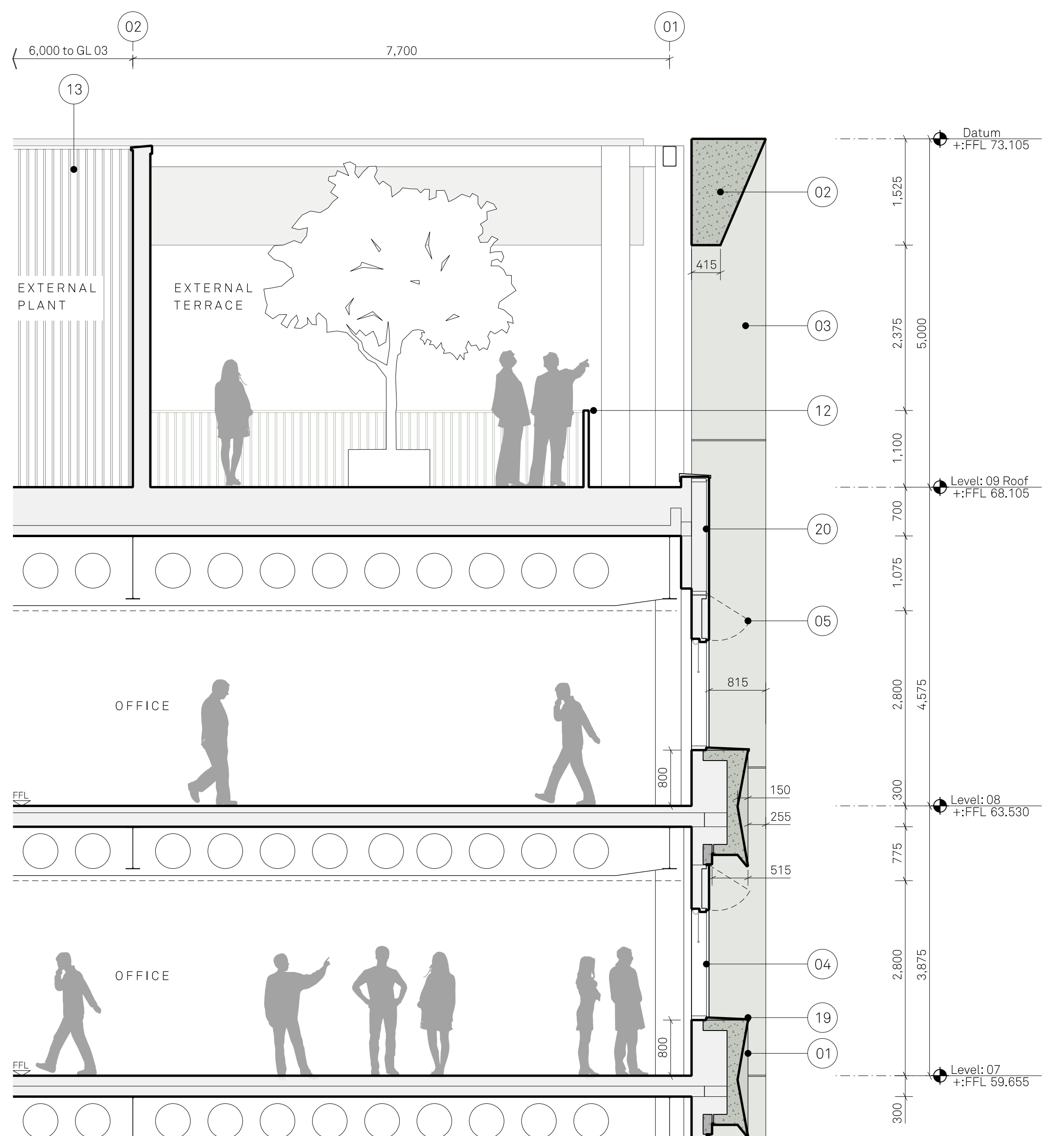
SECTION E Through office & external terrace
