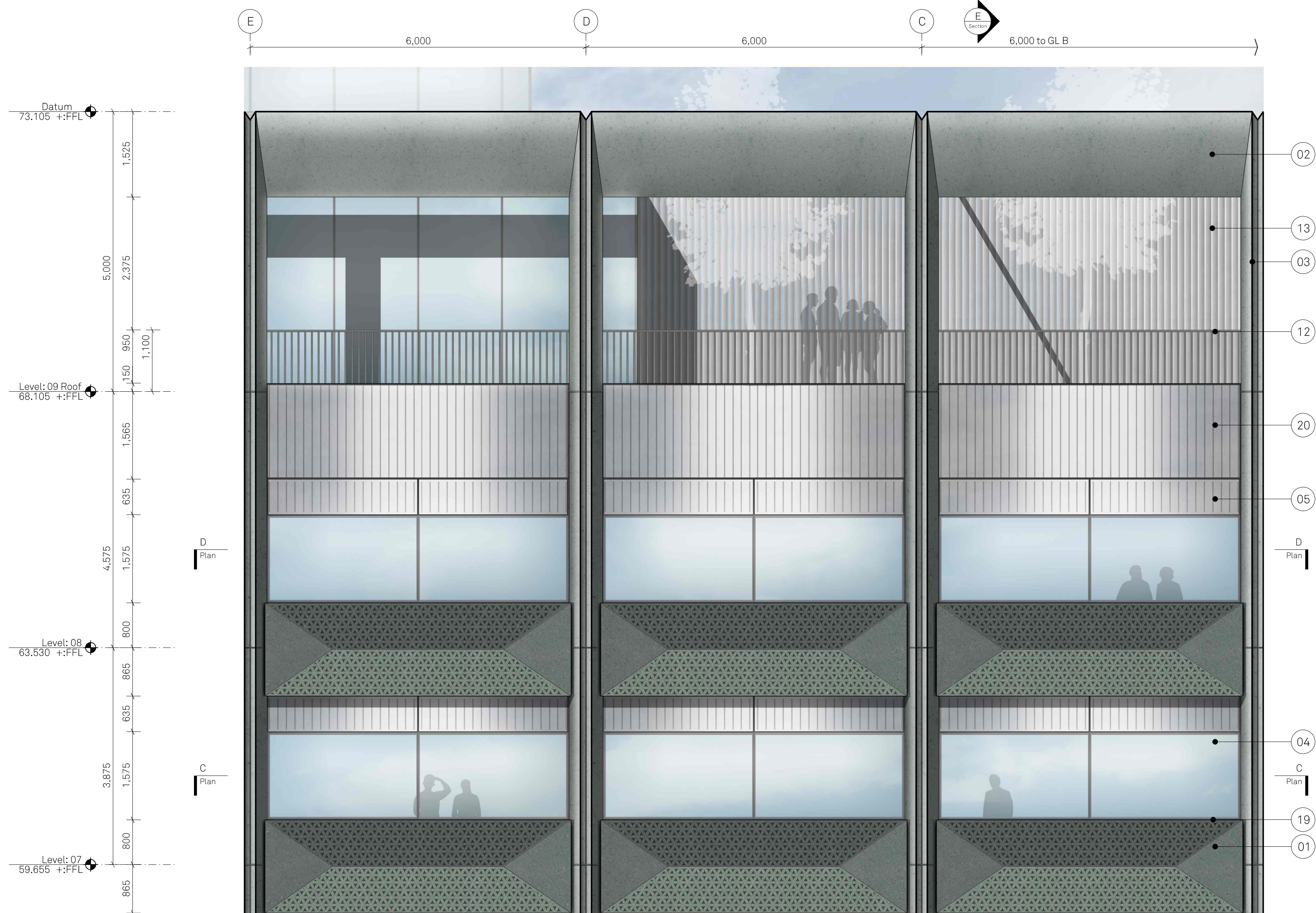
PARTIAL ELEVATION External Terrace
