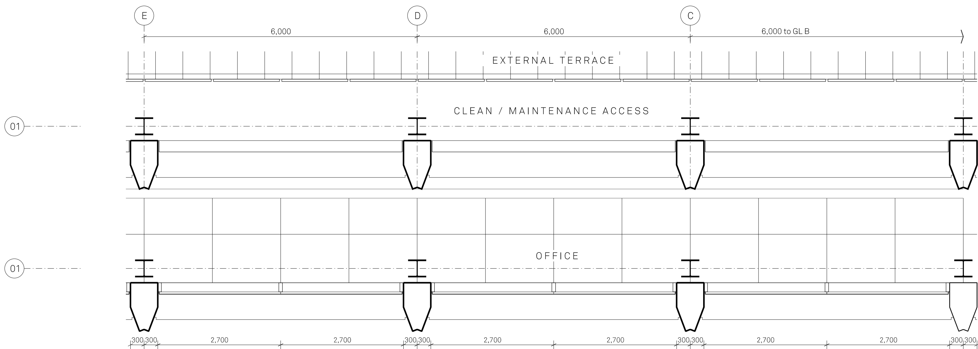
PLAN C & D Typical office & external terrace
