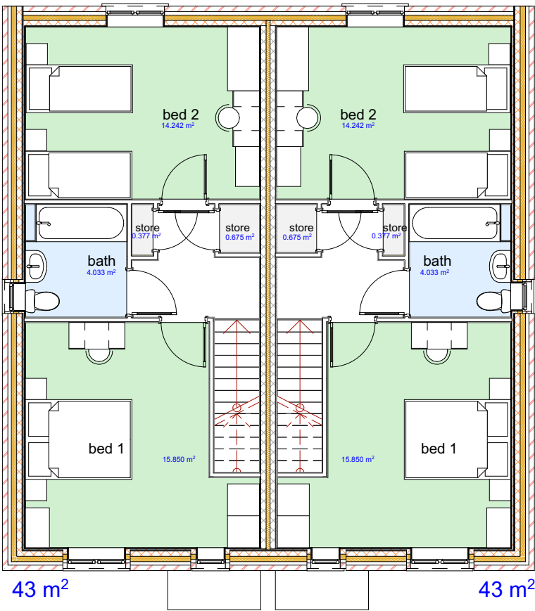
2 01-First Floor 1:100
