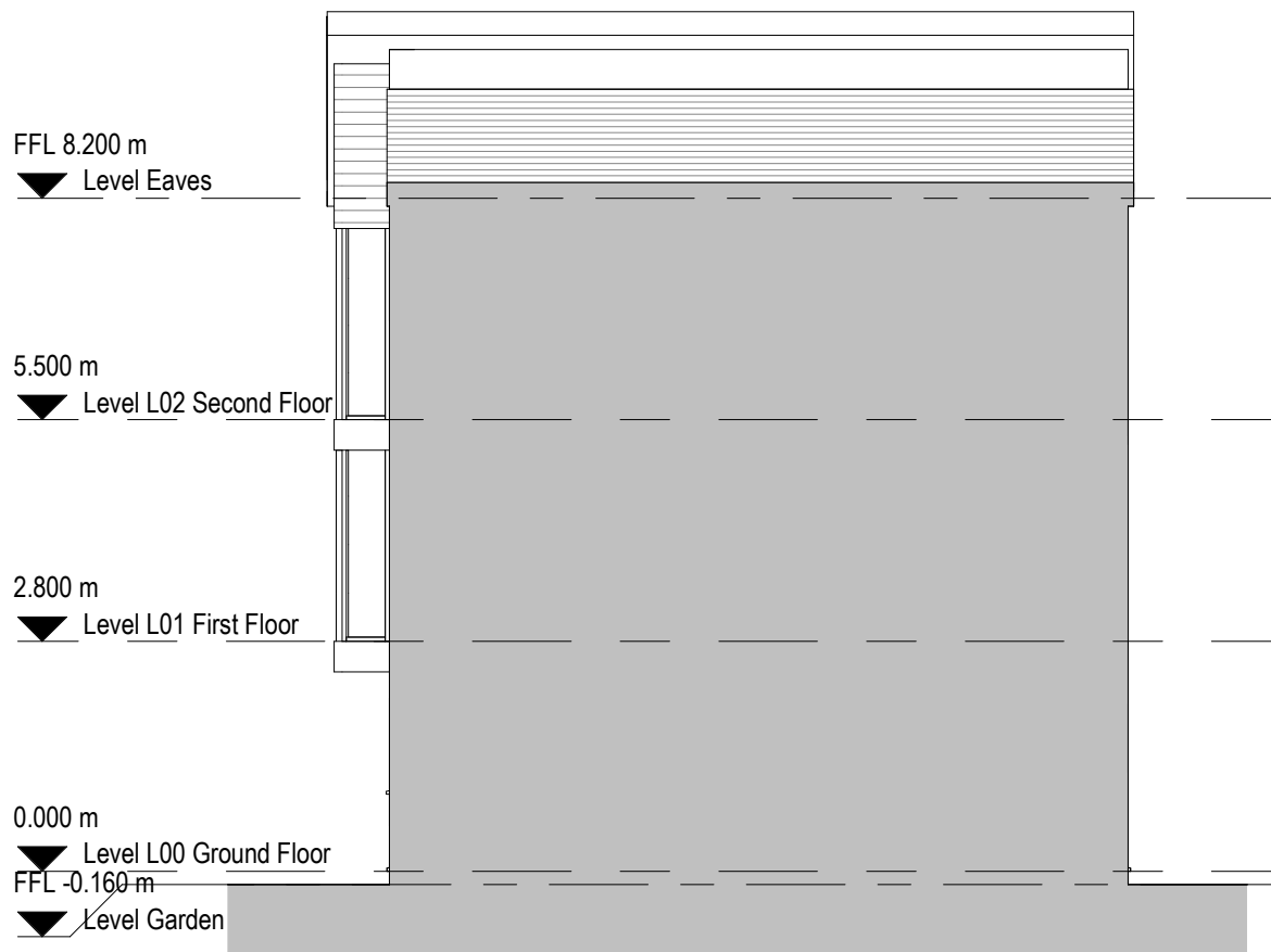
2 Proposed East Elevation 1 : 100
