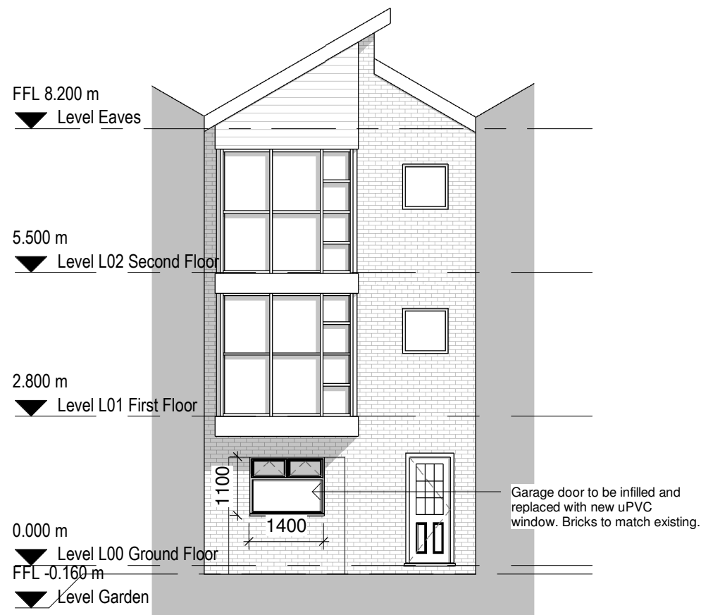
1 Proposed South Elevation 1 : 100
