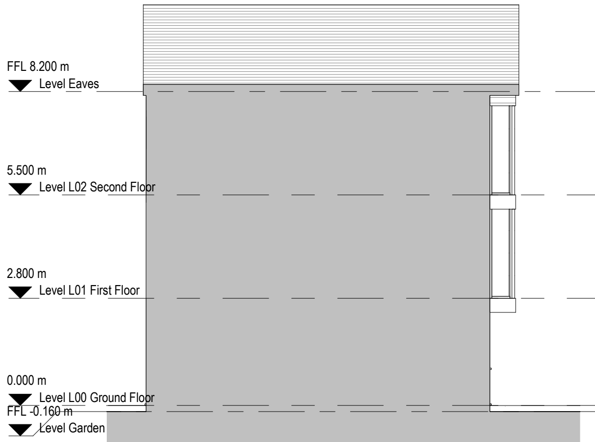
4 Proposed West Elevation 1 : 100
