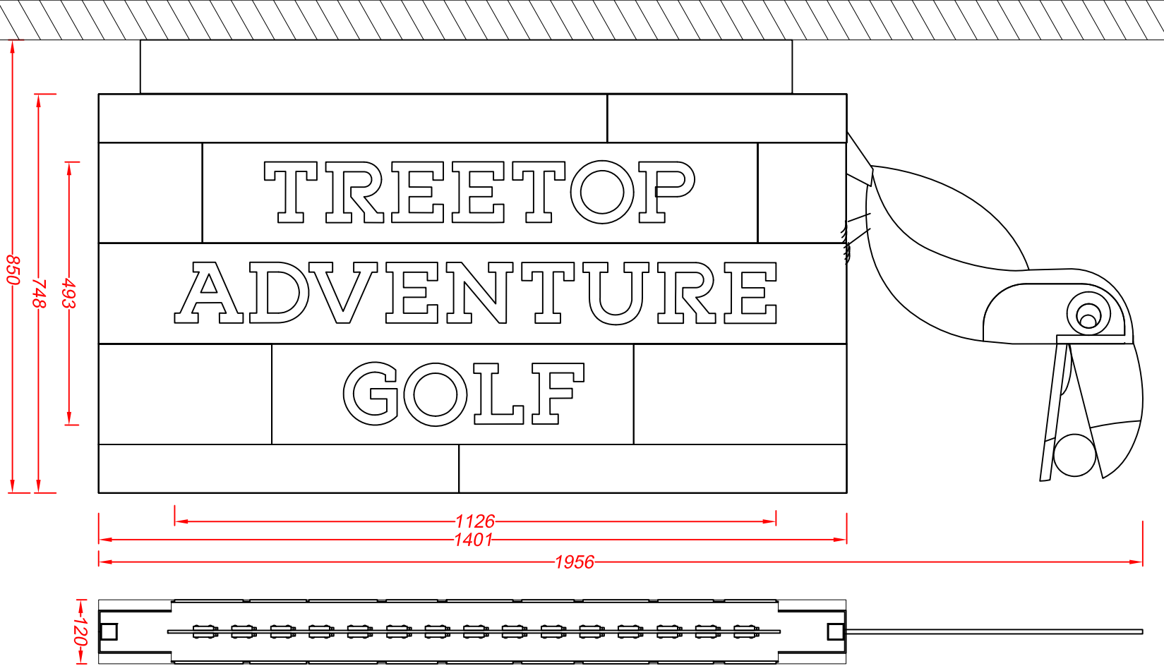
Section A-A through the text Scale 1:10
