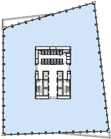
Level 07
