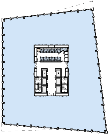
Level 03
