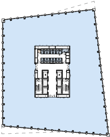
Level 01
