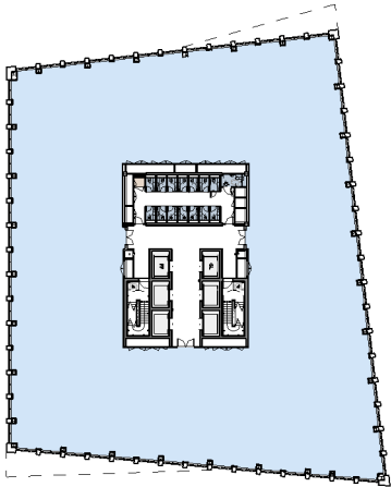
Level 02
