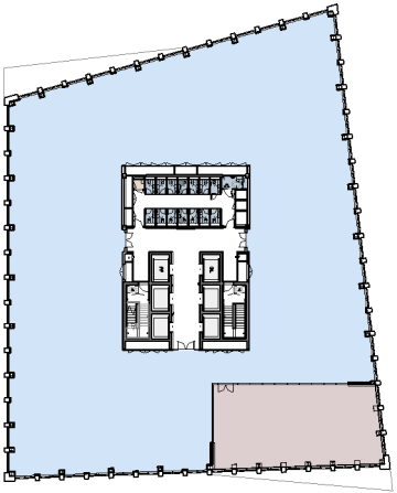
Level 10
