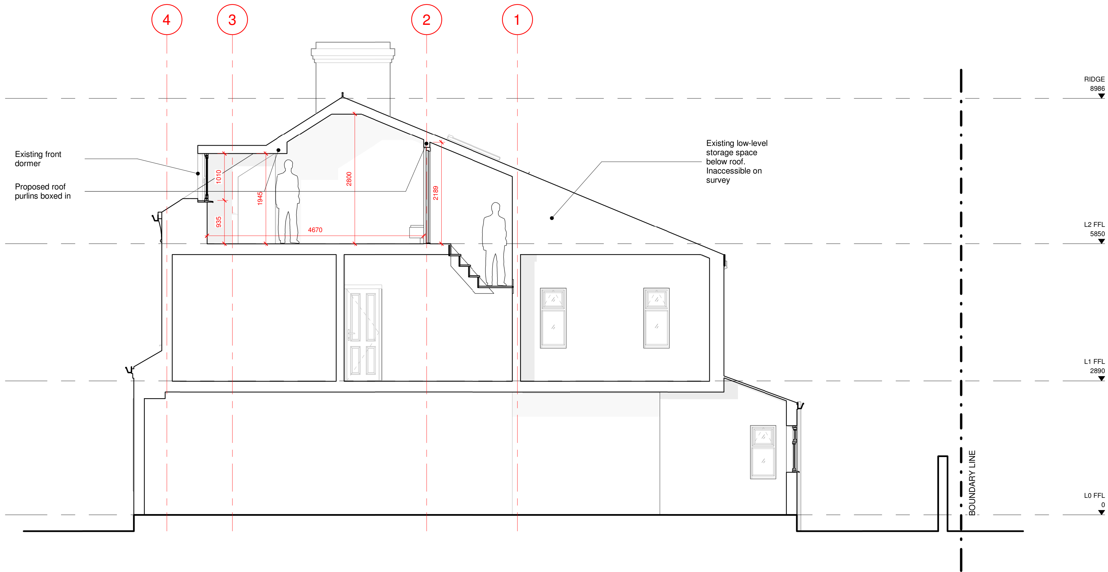
01 EXISTING SECTION AA 1:50
