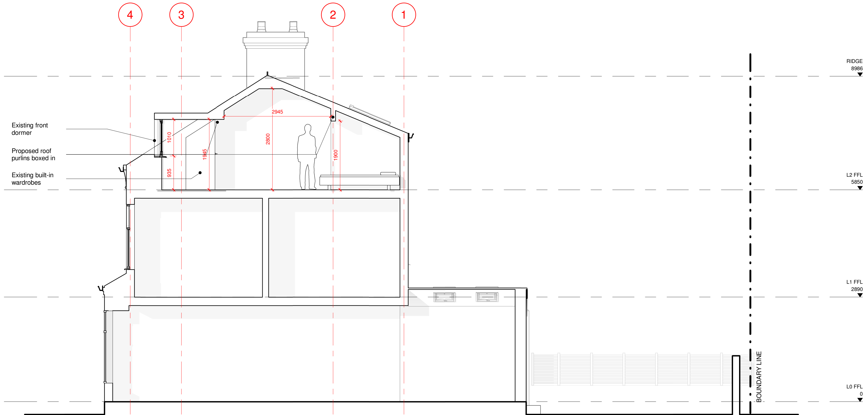
01 EXISTING SECTION AA 1:50
