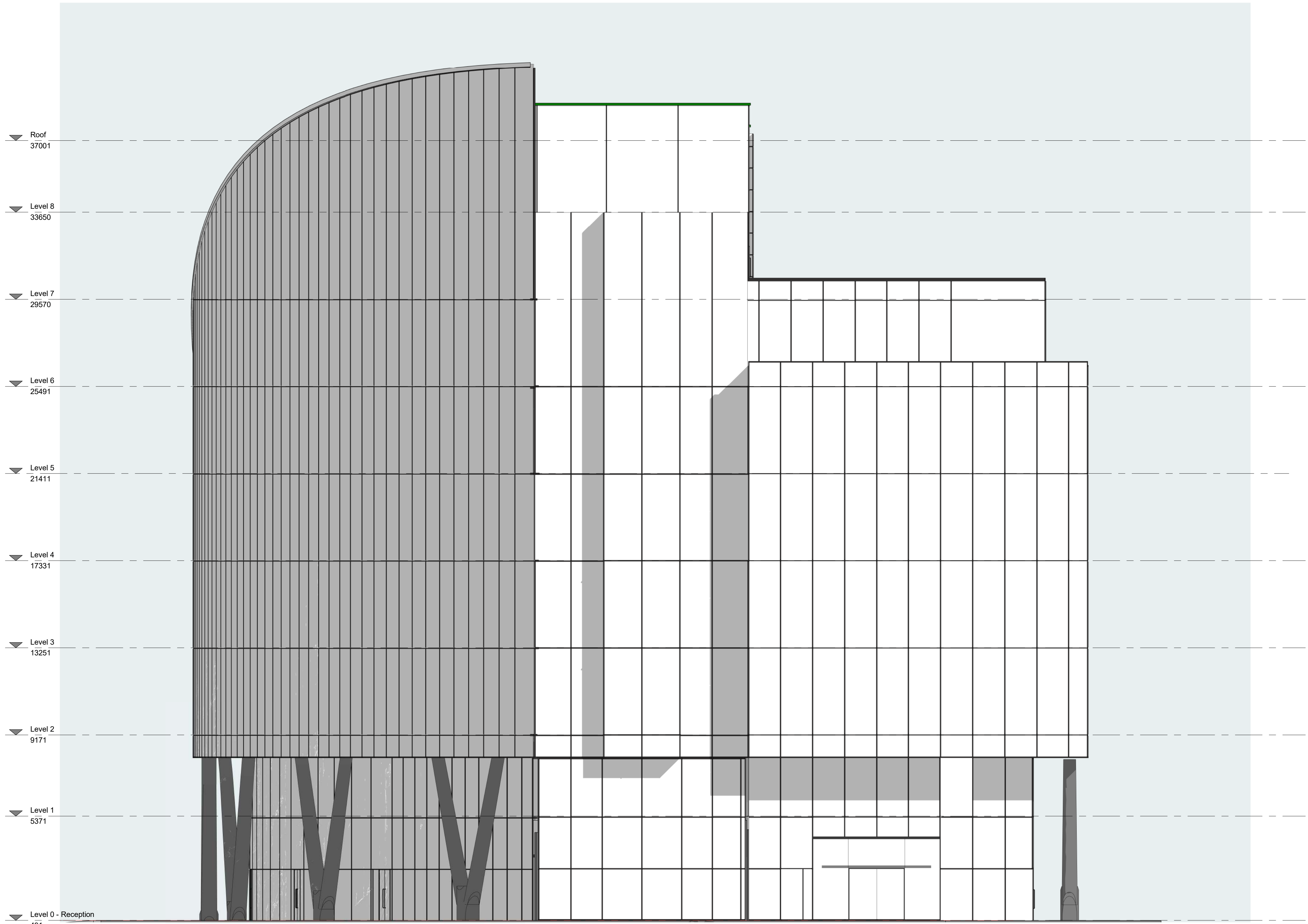
East Elevation - Existing 1 : 100
