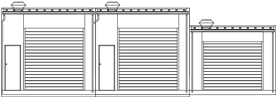
PROPOSED NORTH ELEVATION 1:100
