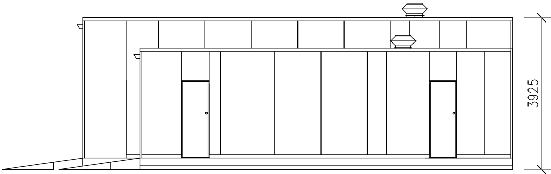
PROPOSED WEST ELEVATION 1:100
