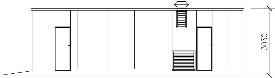
PROPOSED EAST ELEVATION 1:100
