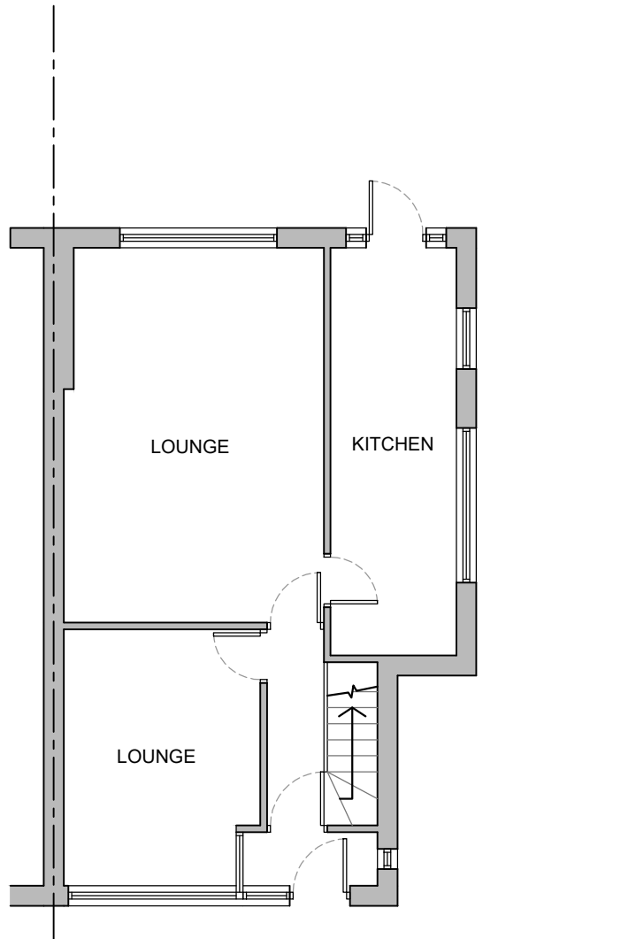
GROUND FLOOR 1:100
