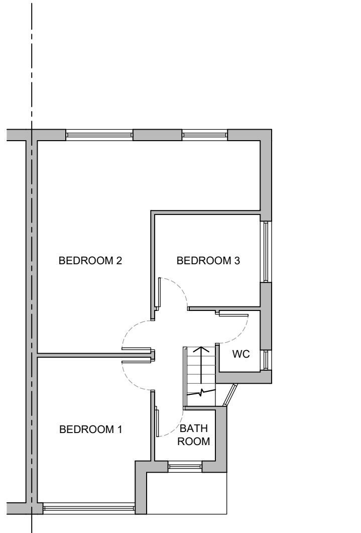
FIRST FLOOR 1:100
