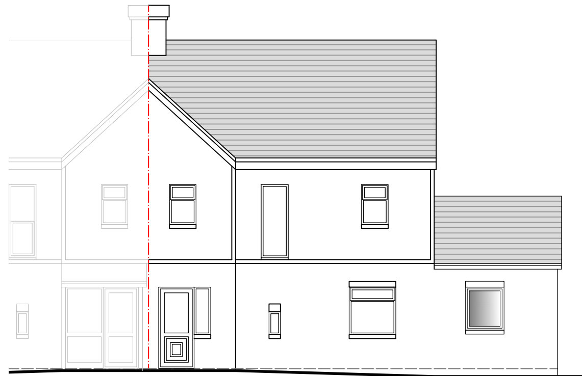
ELEVATION - FRONT
