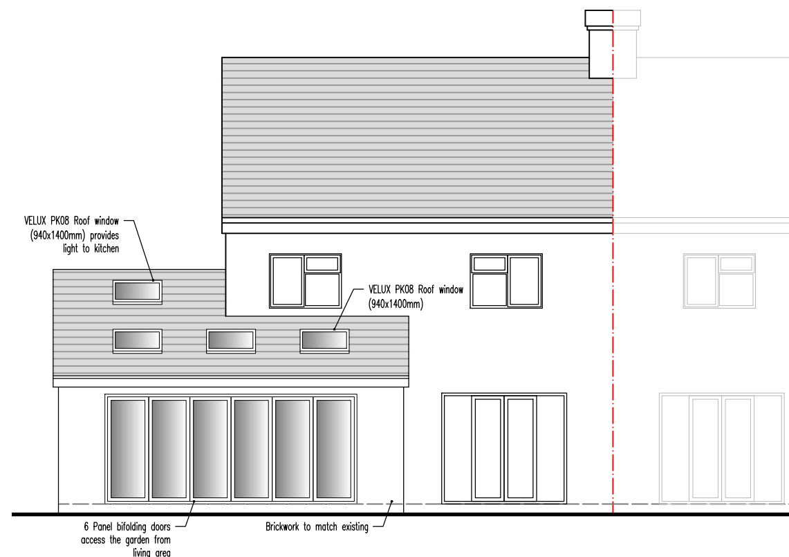
ELEVATION - REAR
