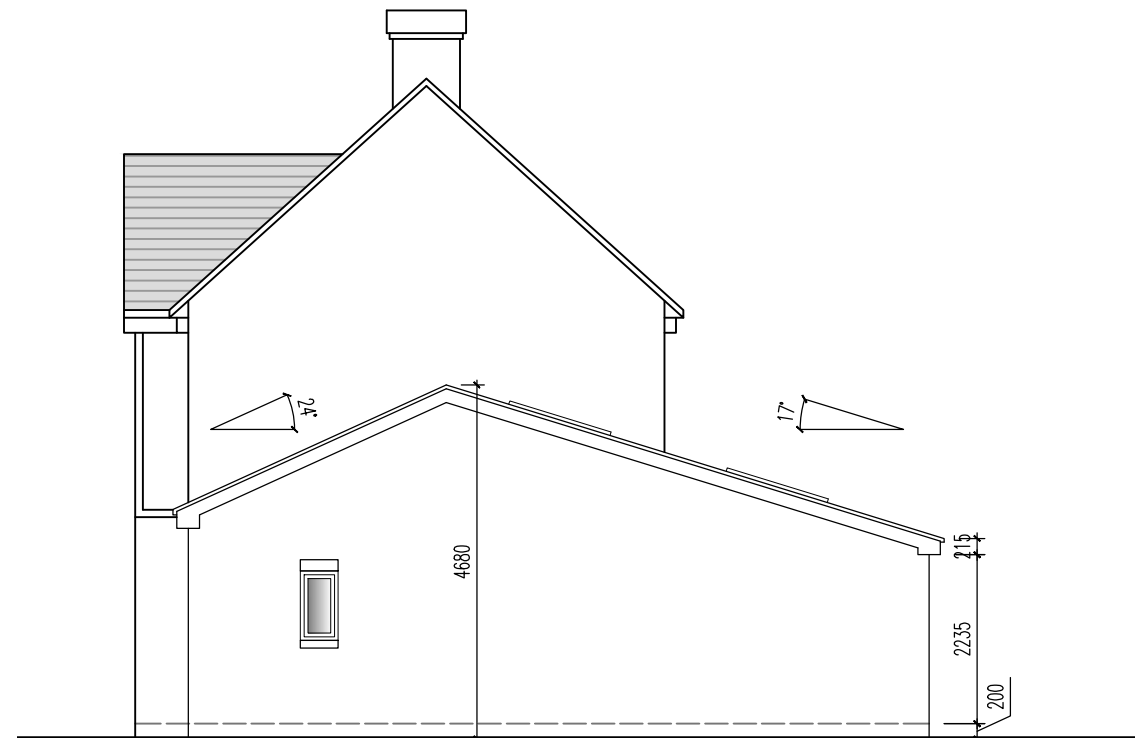
ELEVATION - SIDE 1
