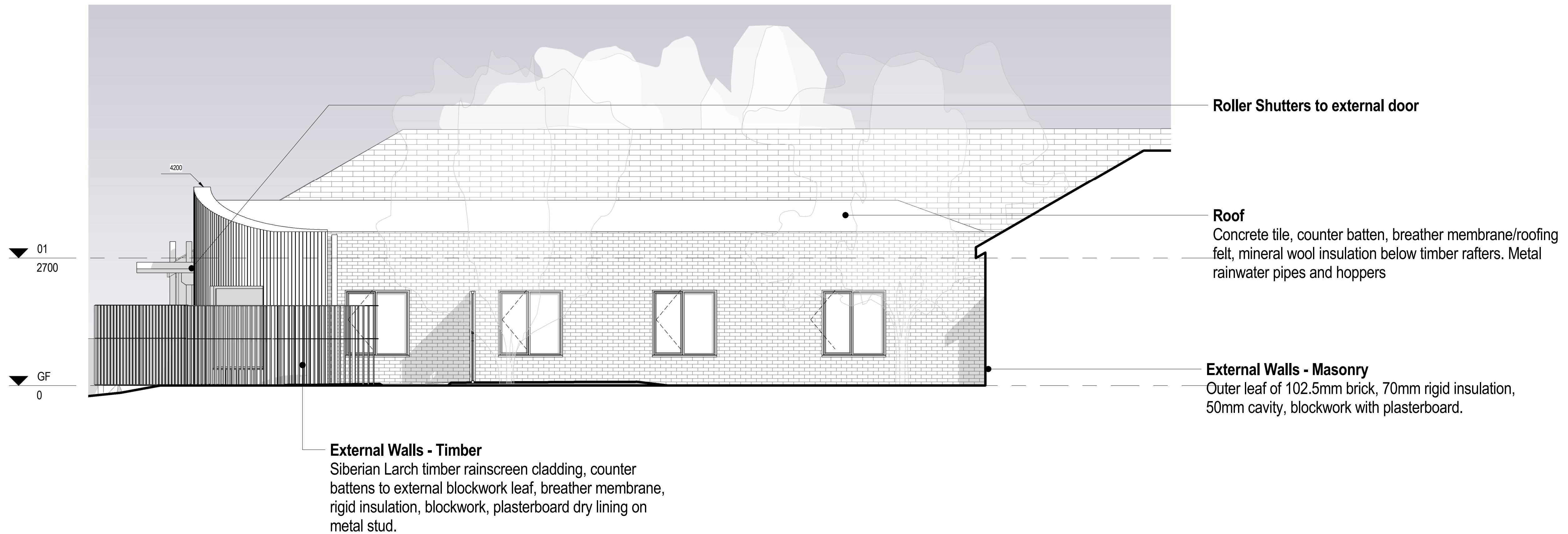
A Option 5 - Elevation A 1 : 50
