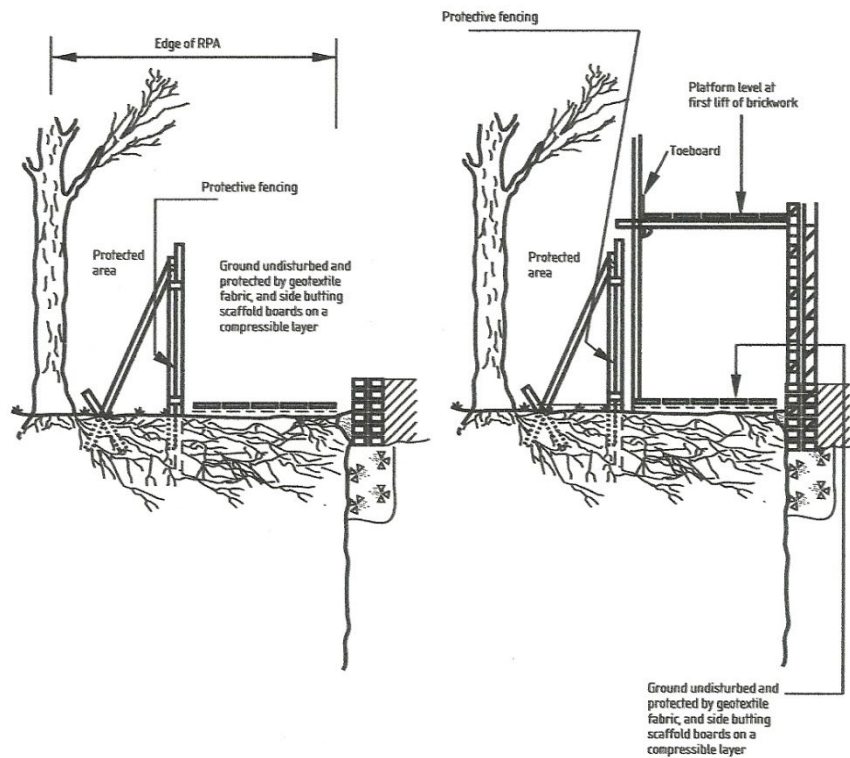
Ground protection and scaffolding within the RPA (taken from BS5837:2005)
