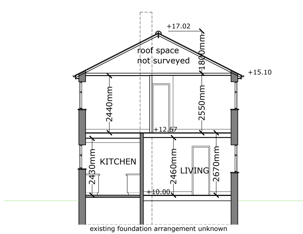
CROSS SECTION
