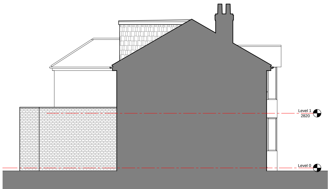
PROPOSED SIDE ELEVATION TOWARDS NO.16
