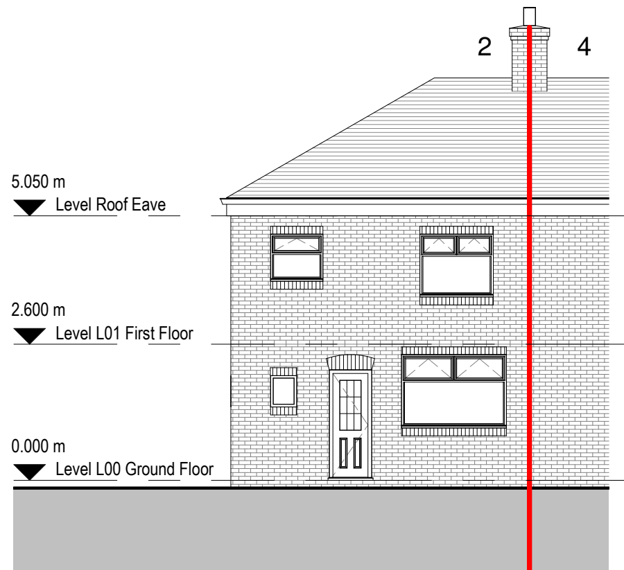
3 Existing West Elevation 1 : 100
