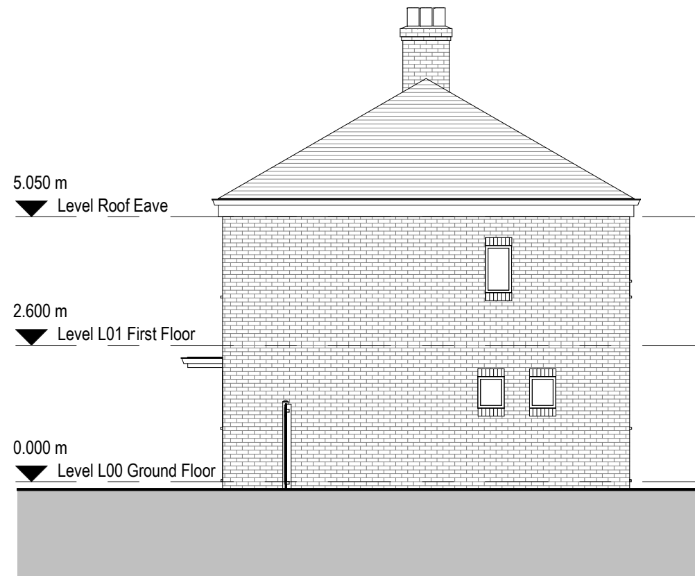
4 Existing North Elevation 1 : 100
