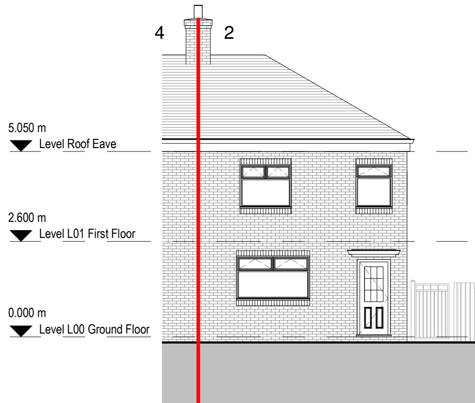
1 Existing East Elevation 1 : 100
