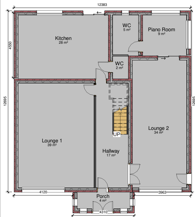
Ground Floor 1 : 100
