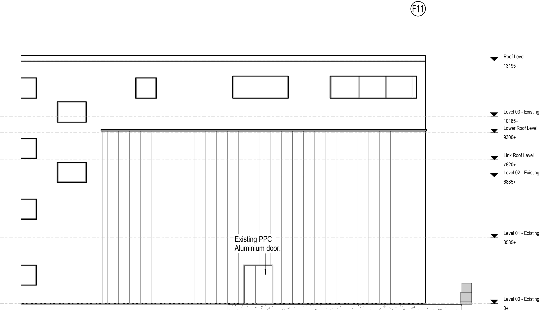
1 | Elevation - North
