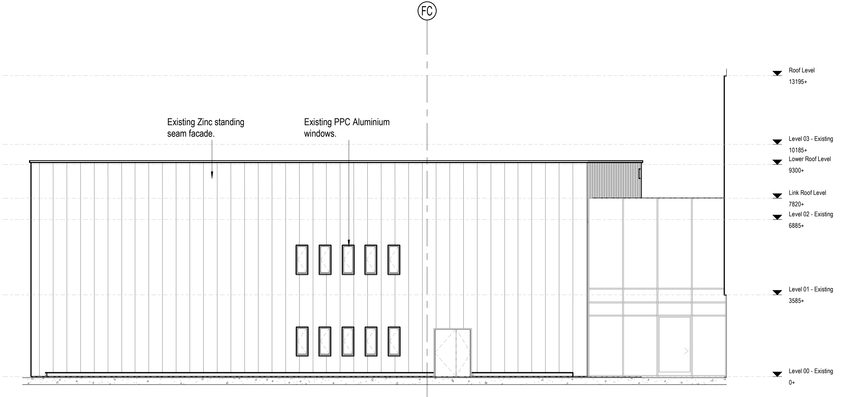
2 | Elevation - West
