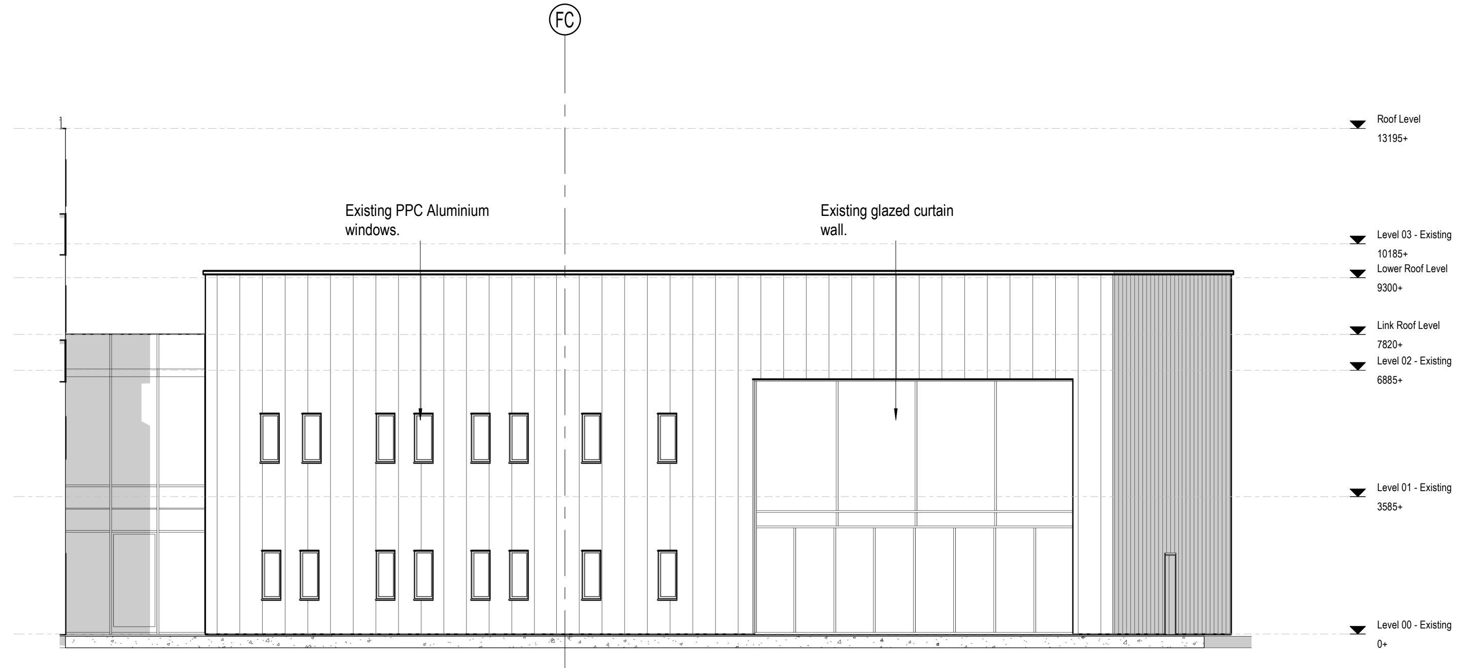
4 | Elevation - East
