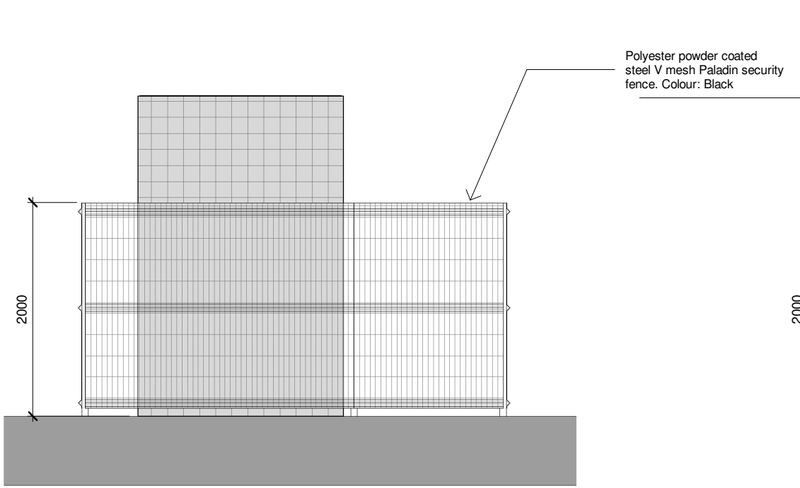
South Inverter South Elevation 1 : 50
