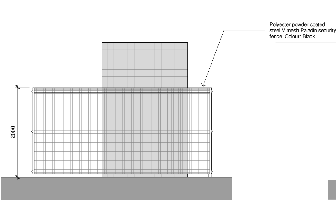
South Inverter North Elevation 1 : 50
