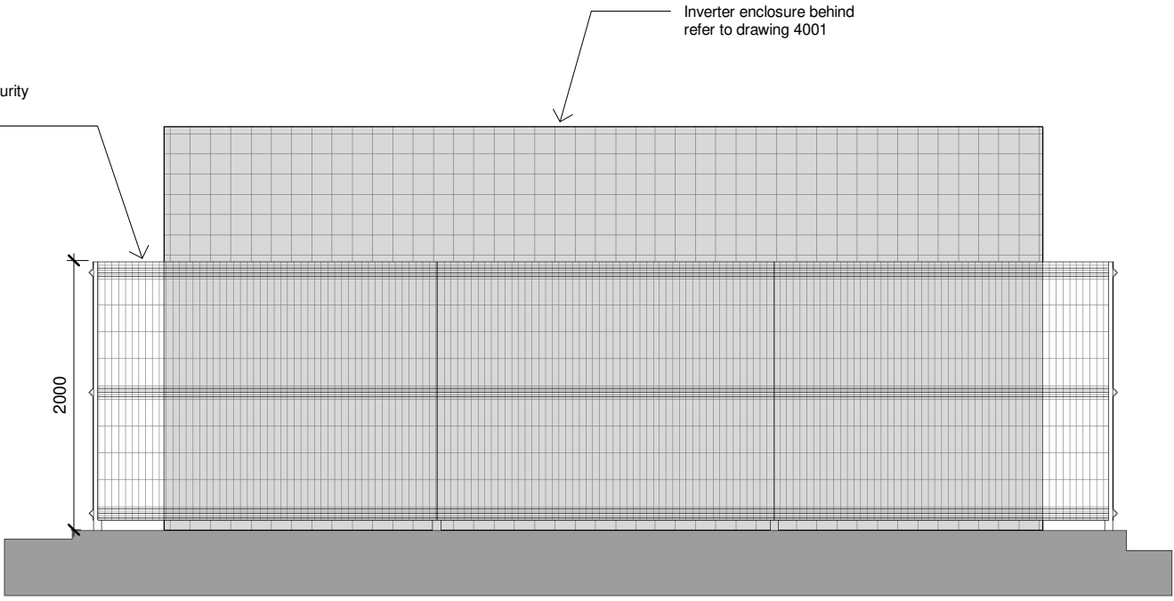
South Inverter East Elevation 1 : 50
