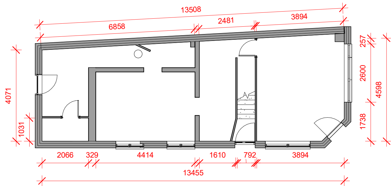
1 Proposed, ground floor, setout 1 : 100
