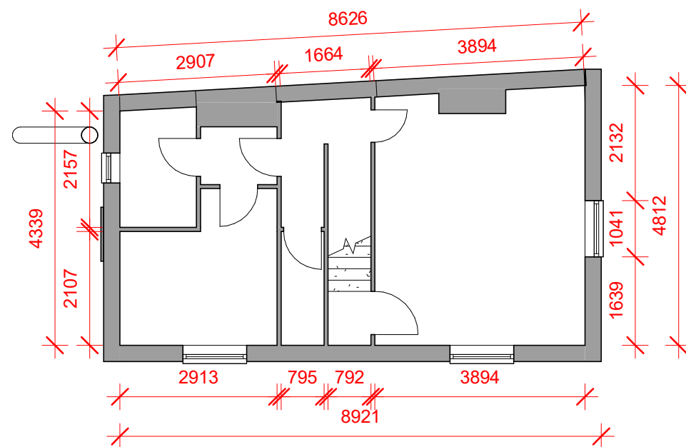
2 Proposed First Floor, setout 1 : 100
