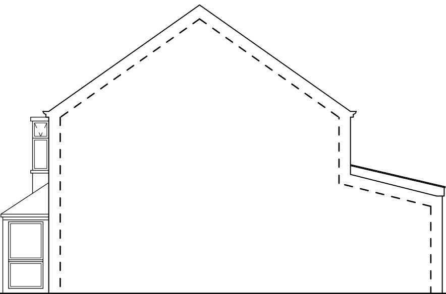
EAST ELEVATION SCALE 1:100 UID - P008
