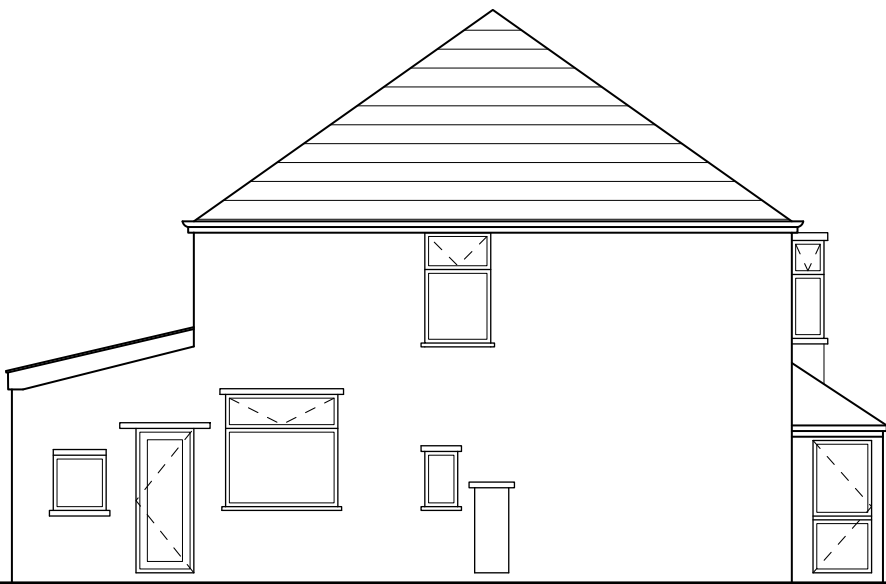
WEST ELEVATION SCALE 1:100 UID - P006
