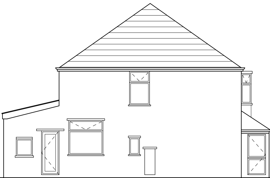
WEST ELEVATION SCALE 1:100 UID - E006
