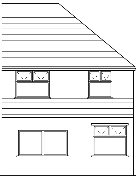
NORTH ELEVATION SCALE 1:100 UID - E007
