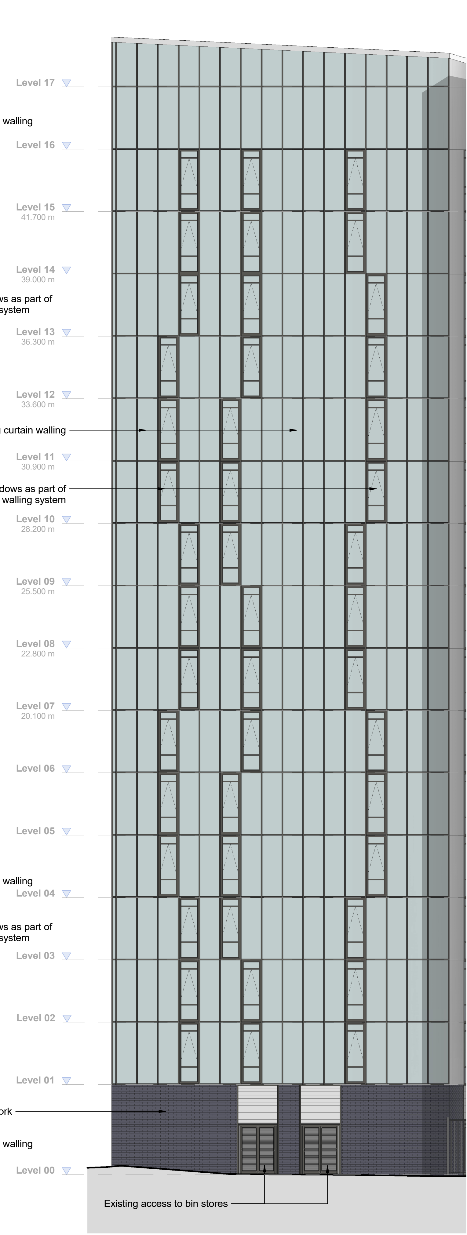
2 Block 2 Existing GA East Elevation 1 : 100
