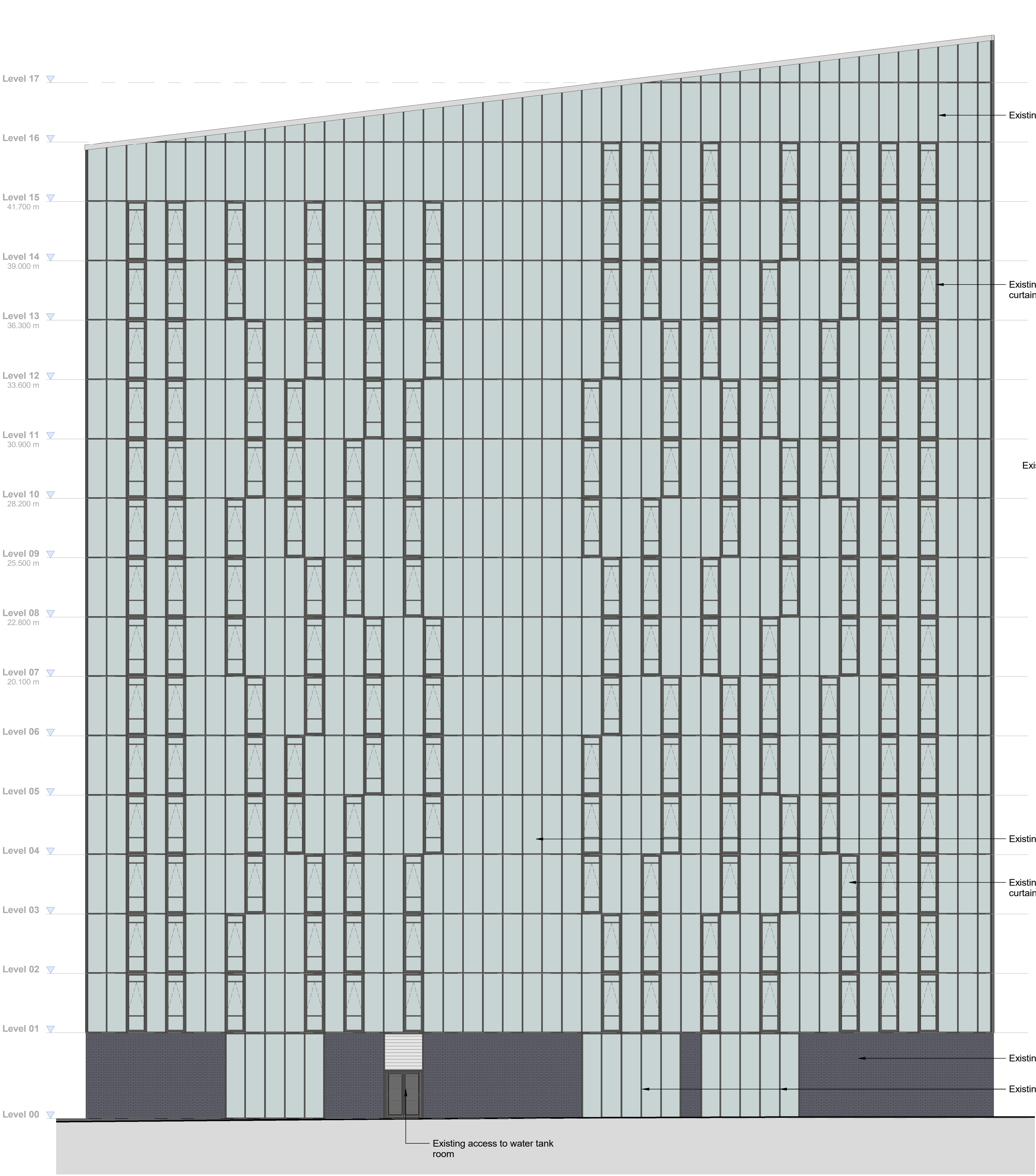
1 Block 2 Existing GA South Elevation 1 : 100
