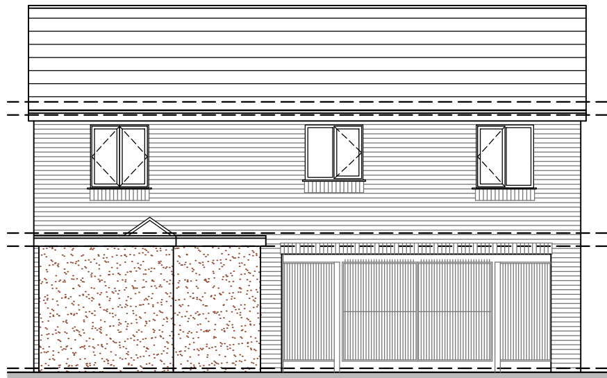
REAR ELEVATION 1:100
