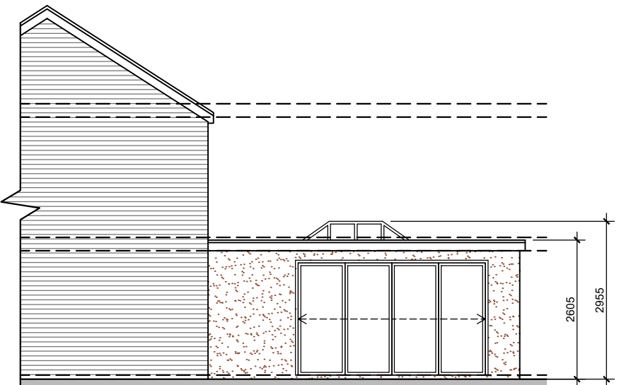
SIDE ELEVATION 1:100
