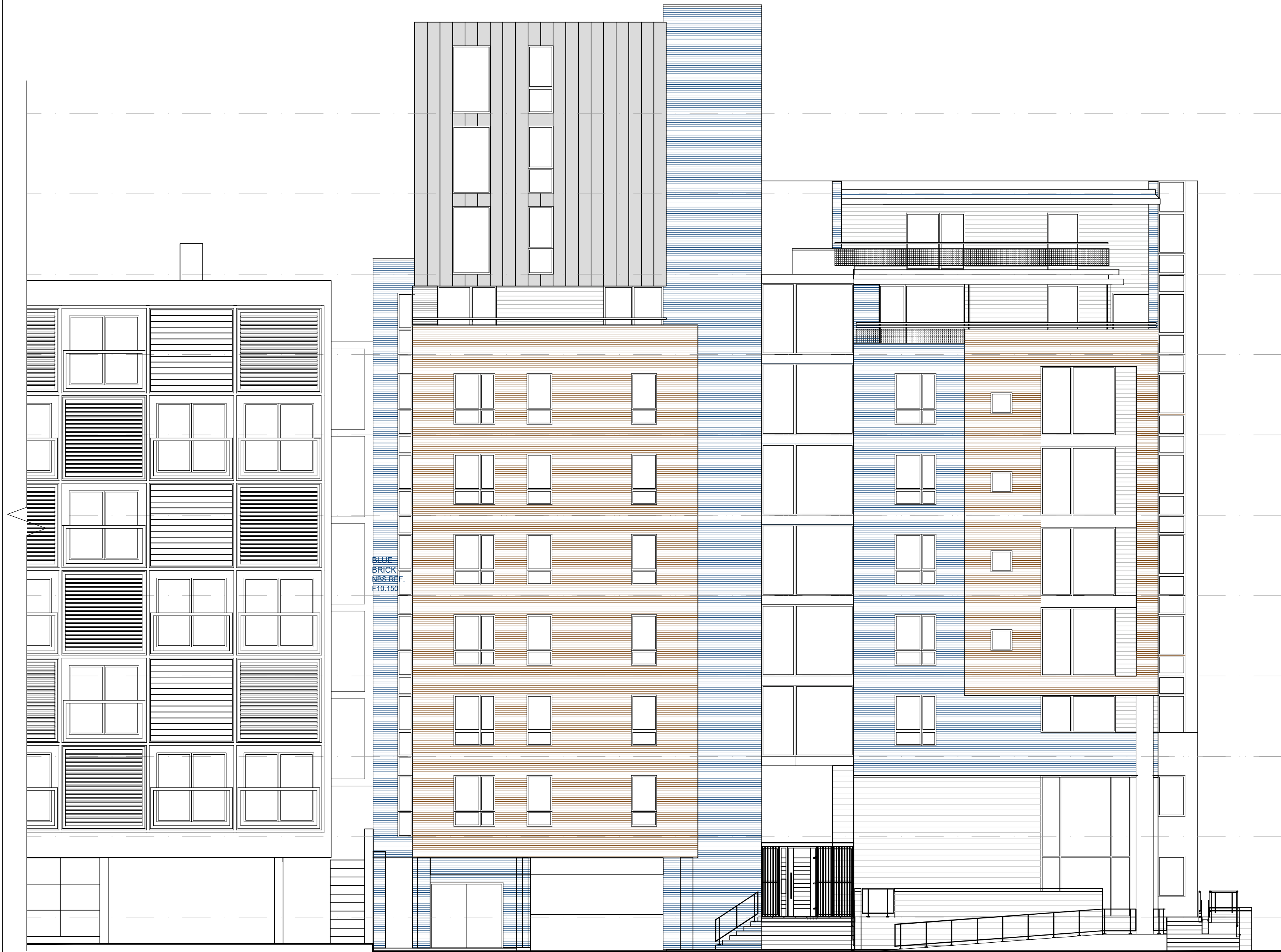
Existing Elevation 3 Arundel Street 1:100
