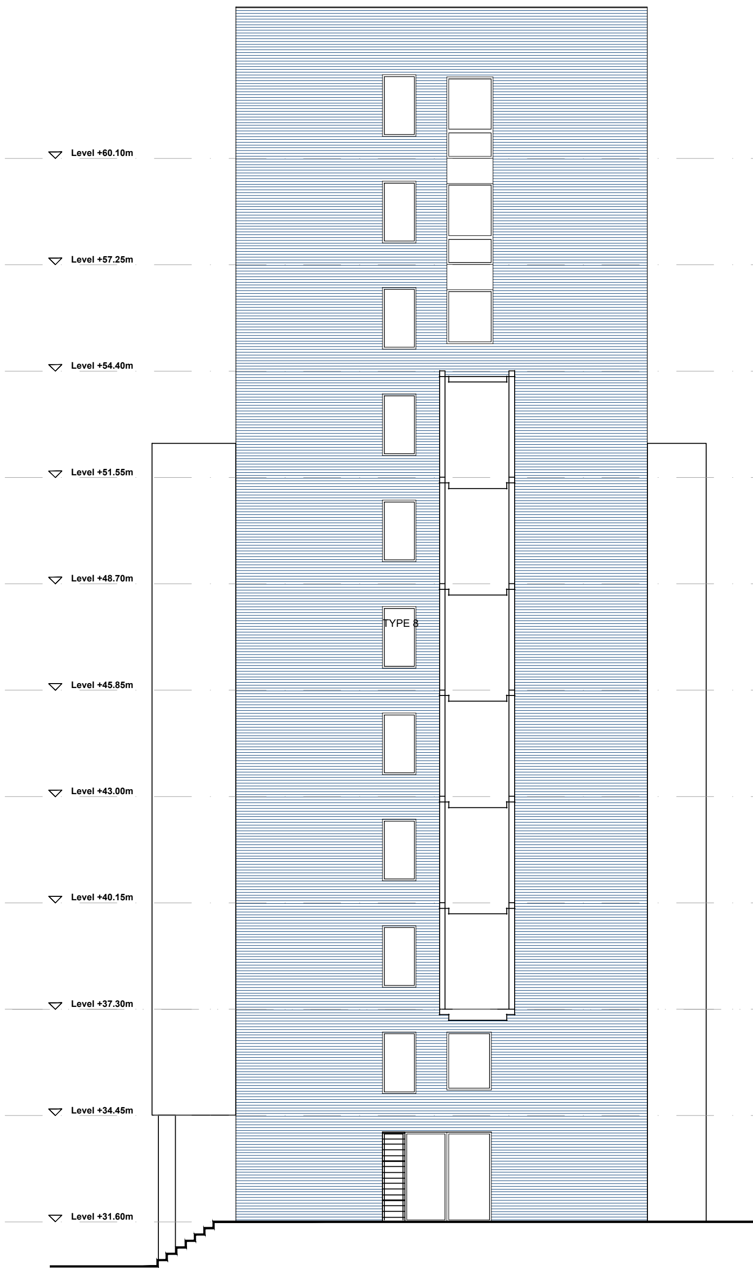
Existing Elevation 4 Arundel Street Tower North 1:100
