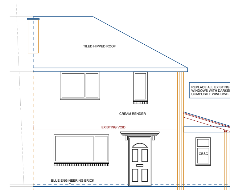
PROPOSED FRONT ELEVATION - SECTION
