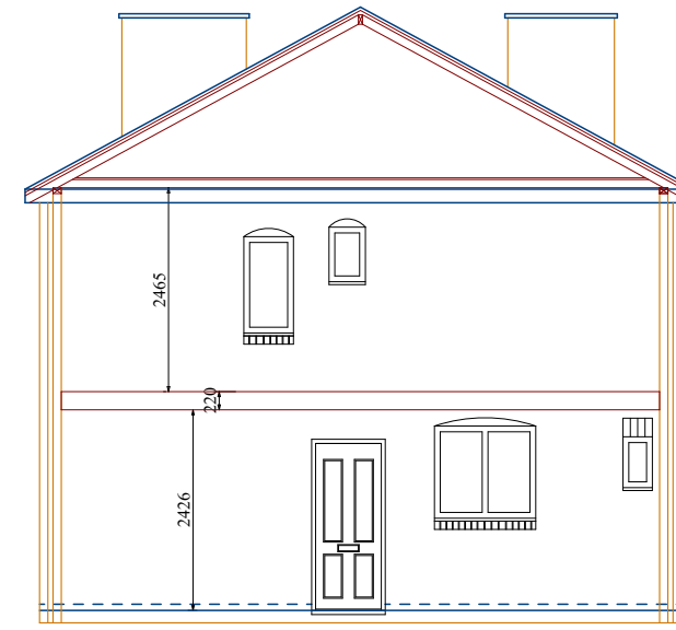
EXISTING RIGHT SIDE SECTION
