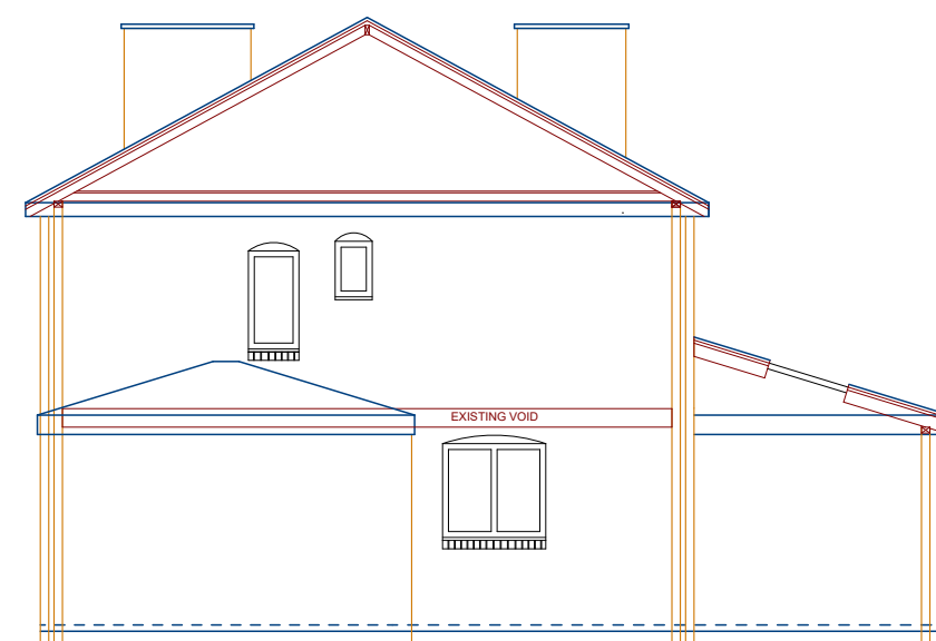
PROPOSED RIGHT SIDE SECTION
