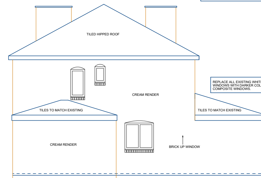
PROPOSED RIGHT SIDE ELEVATION
