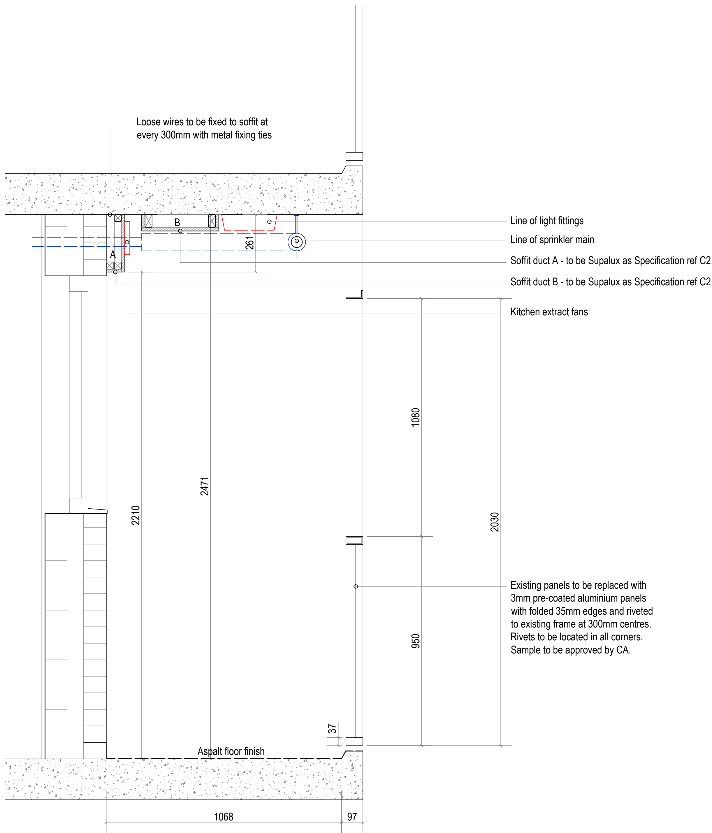
Section through high level walkway
