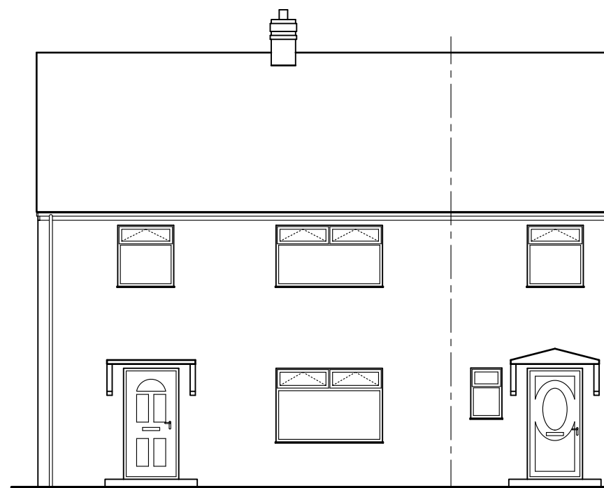
FRONT ELEVATION AS EXISTING
