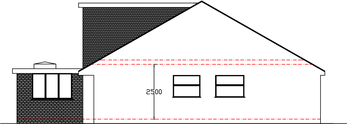
Elevation From No 7
