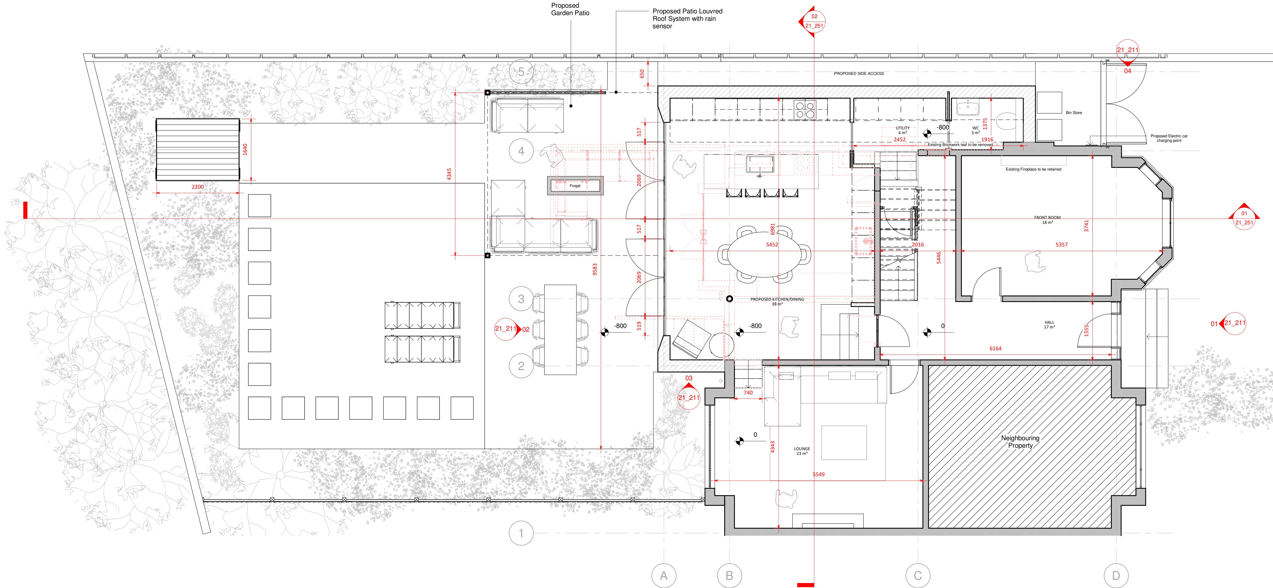
01 PROPOSED L0 PLAN 1 : 50
