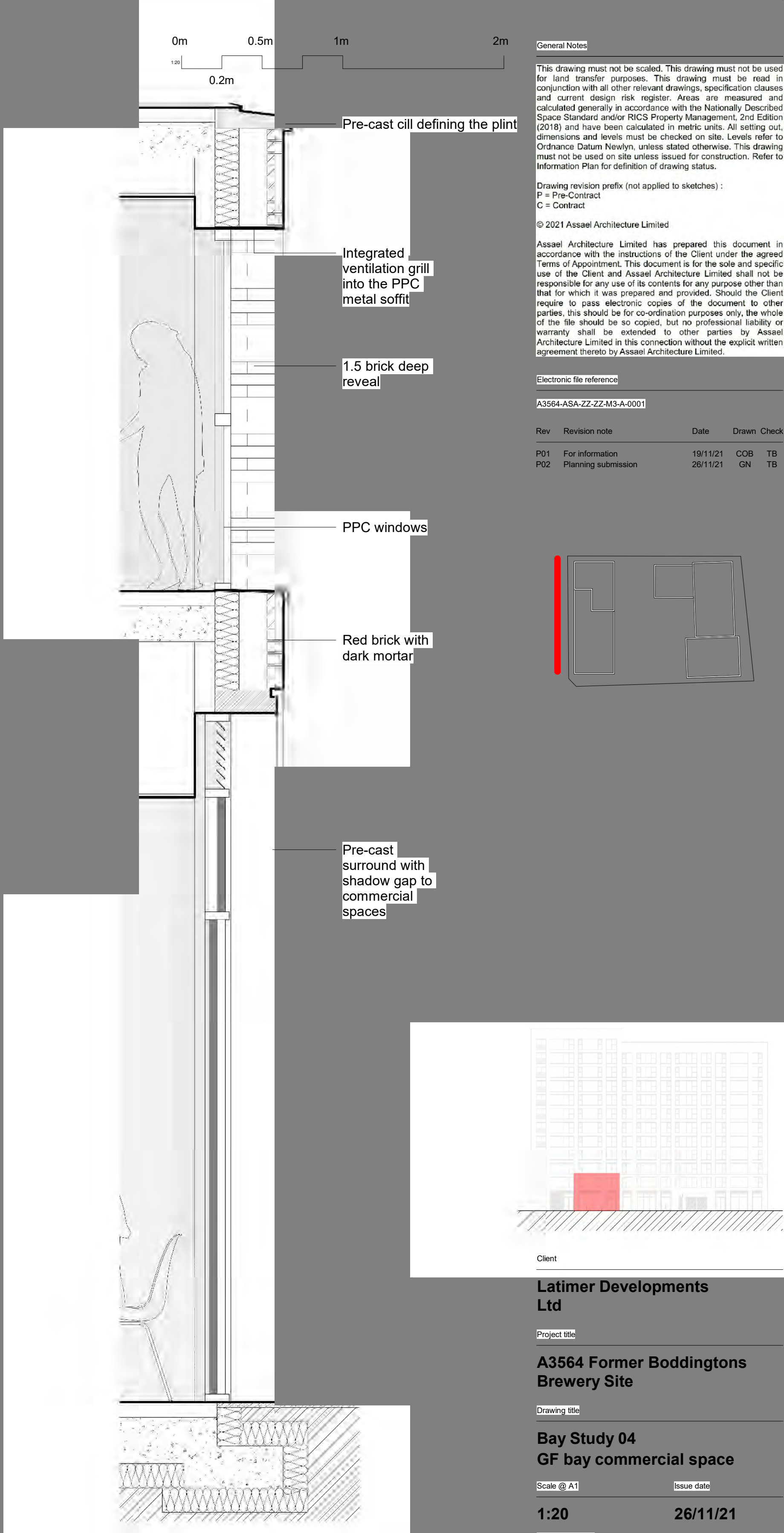
2 Bay Study 04 - Section Scale: 1 : 20
